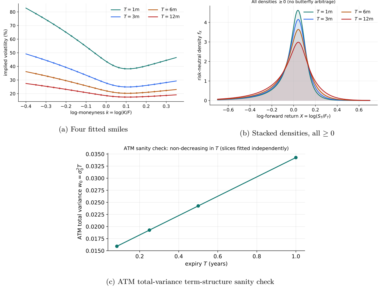
Figure 1: The per-slice no-butterfly guarantee, produced end to end by the production LQD fitter on a synthetic calendar-monotone surface (panels a, b), plus an ATM term-structure sanity check on independently fitted slices (panel c). Full-strike calendar-arbitrage control is Note 10's subject.
