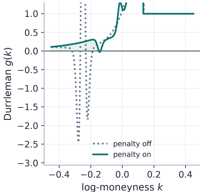
B penalty on: pulled back to admissible
