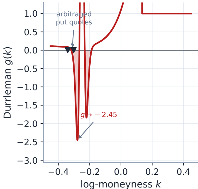
A penalty off: a hat chases the kink
