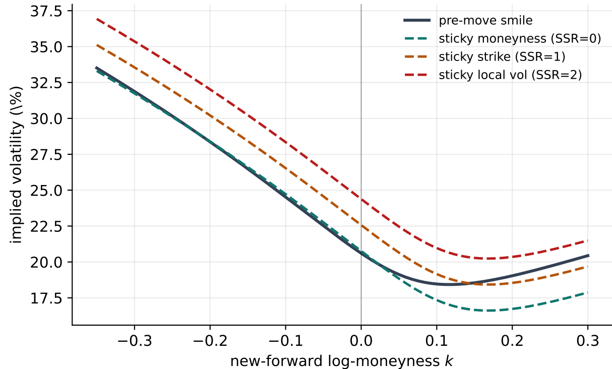
Smile after a -5\% spot move
