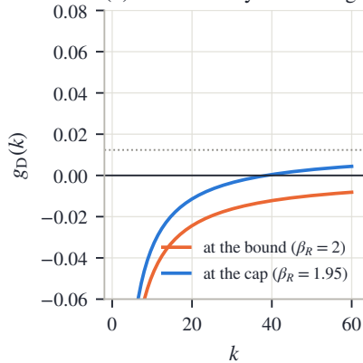
(b) the boundary carries negative density (c) the moment budget collapses at the cap
