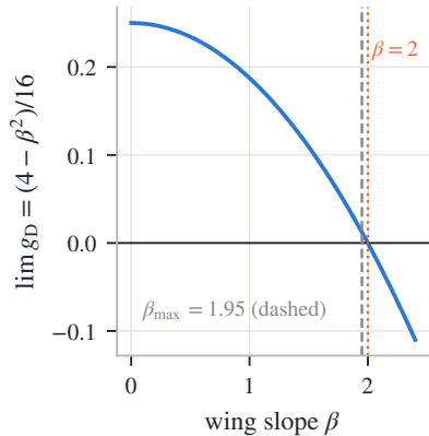
(a) the tail limit changes sign at 2
