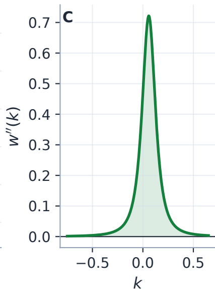
strict convexity: w'' > 0
