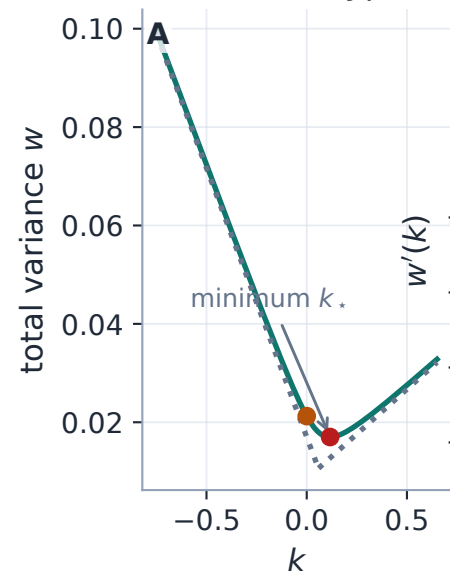
one rounded hyperbola
