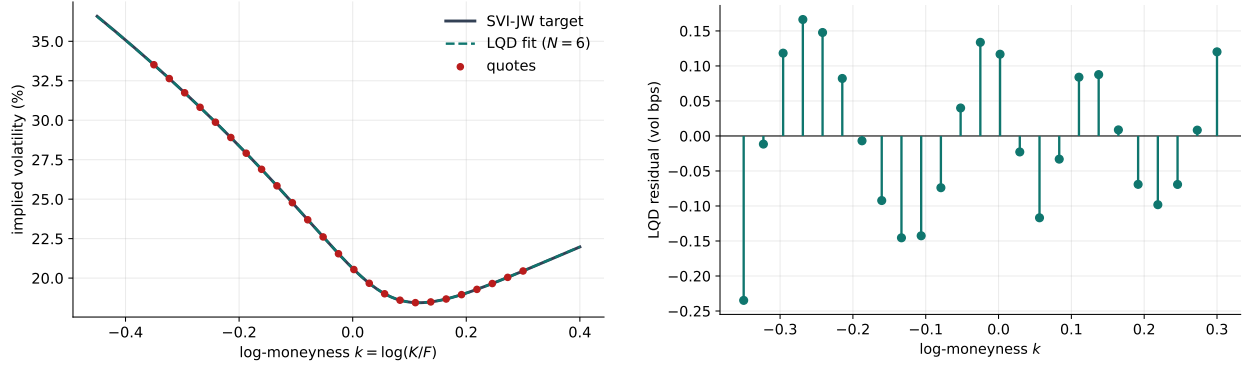
Figure 1: Left: the SVI-JW target, the seven-parameter LQD fit, and the quotes. Right: the LQD implied-volatility residual at the quotes, in volatility basis points. Beyond the calibration window the LQD curve is its own Lee-consistent extrapolation, not an SVI continuation.
