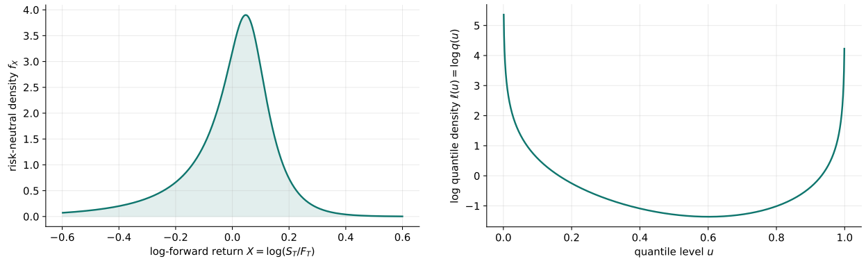
Figure 2: Left: the risk-neutral log-return density implied by the SVI fit — non-negative by construction. Right: the fitted log quantile density \ell(u) = \log q(u) ; the -\log u - \log(1 - u) endpoints are the source of the exponential tails.
