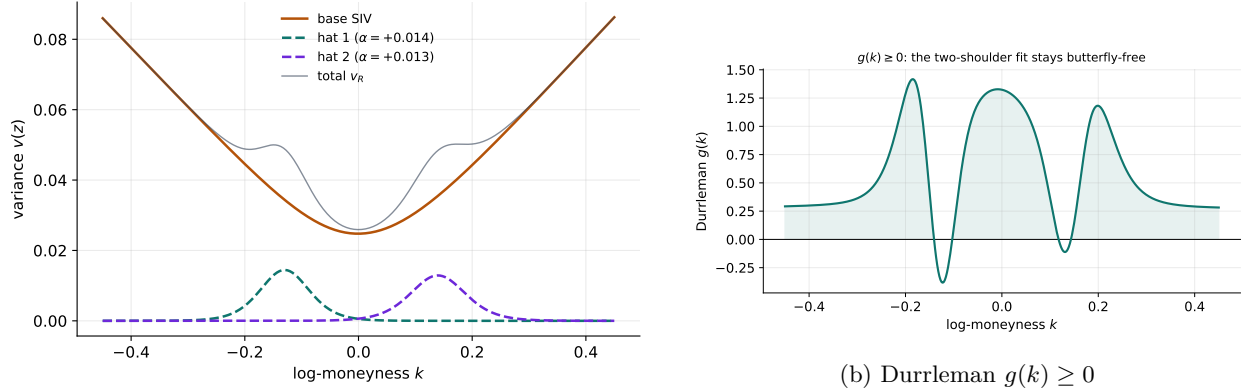
Figure 2: Left: the additive decomposition — the convex base owns the wings, the hats own the shoulders. Right: the butterfly diagnostic stays non-negative.
