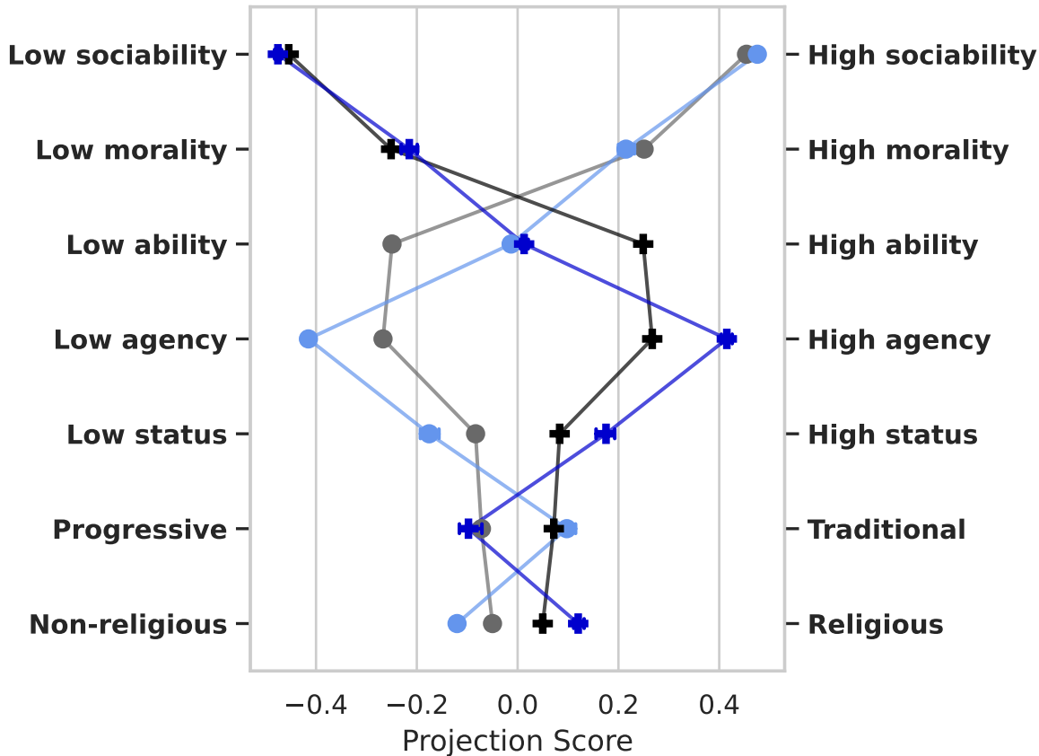
Apertus-8B-Instruct-2509, Default vs Democratic
