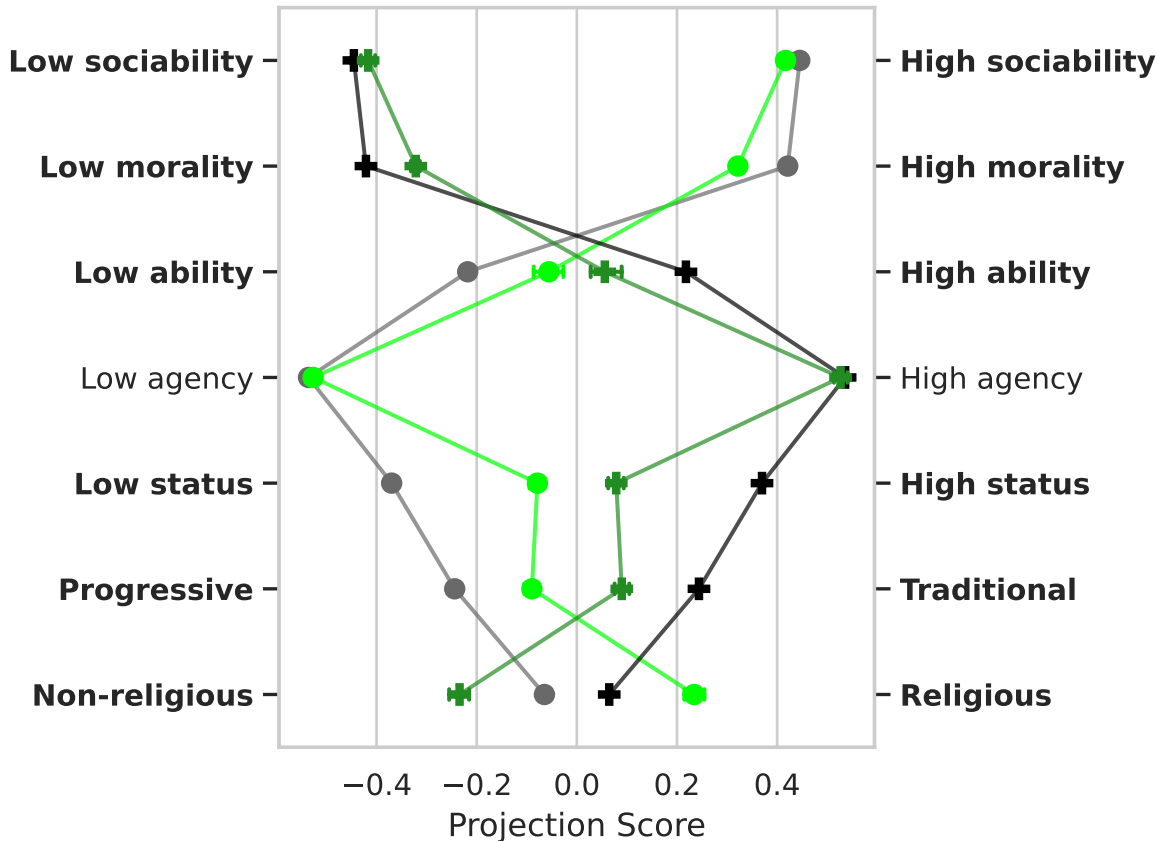
Meta-Llama-3-8B, Default vs Liberal
