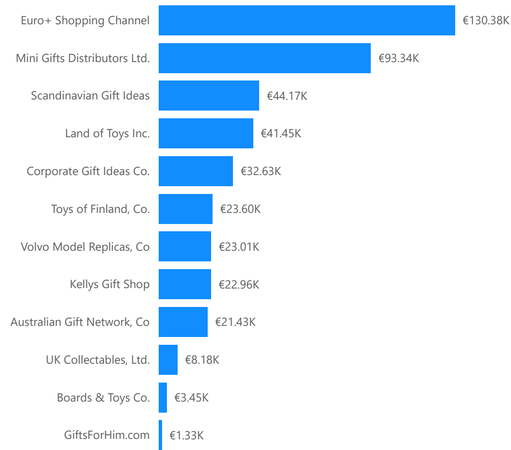
Amount by Customer
