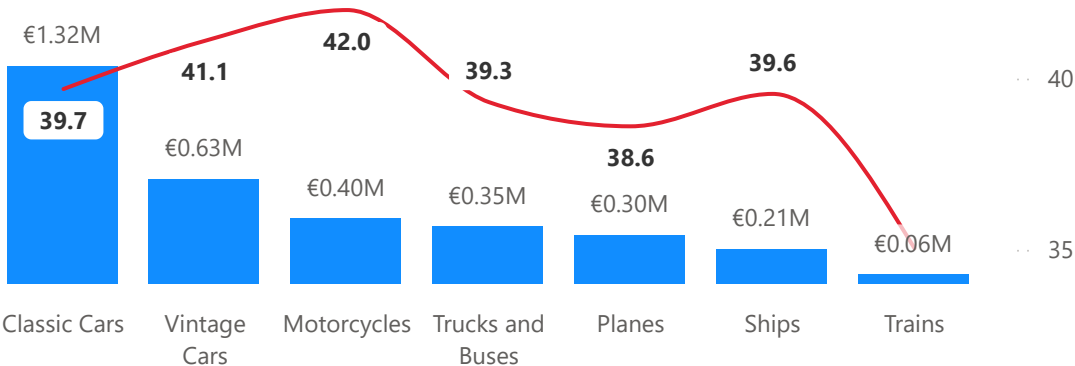
Margin Net and % by Category
