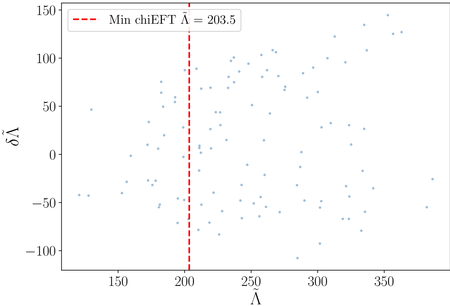
GW170817 BNS Default ( \log L \lesssim 556.8 )
