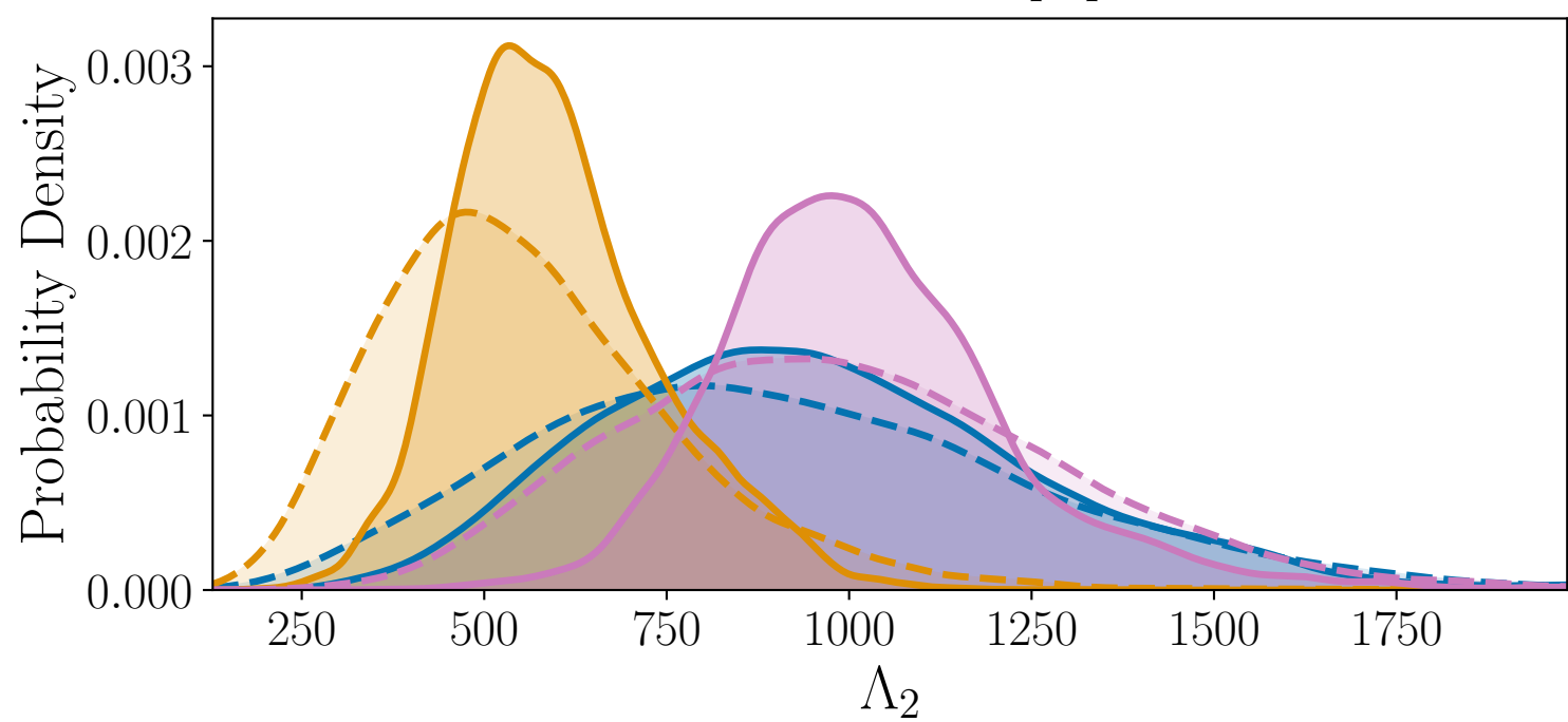
GW230529 - Gaussian population
