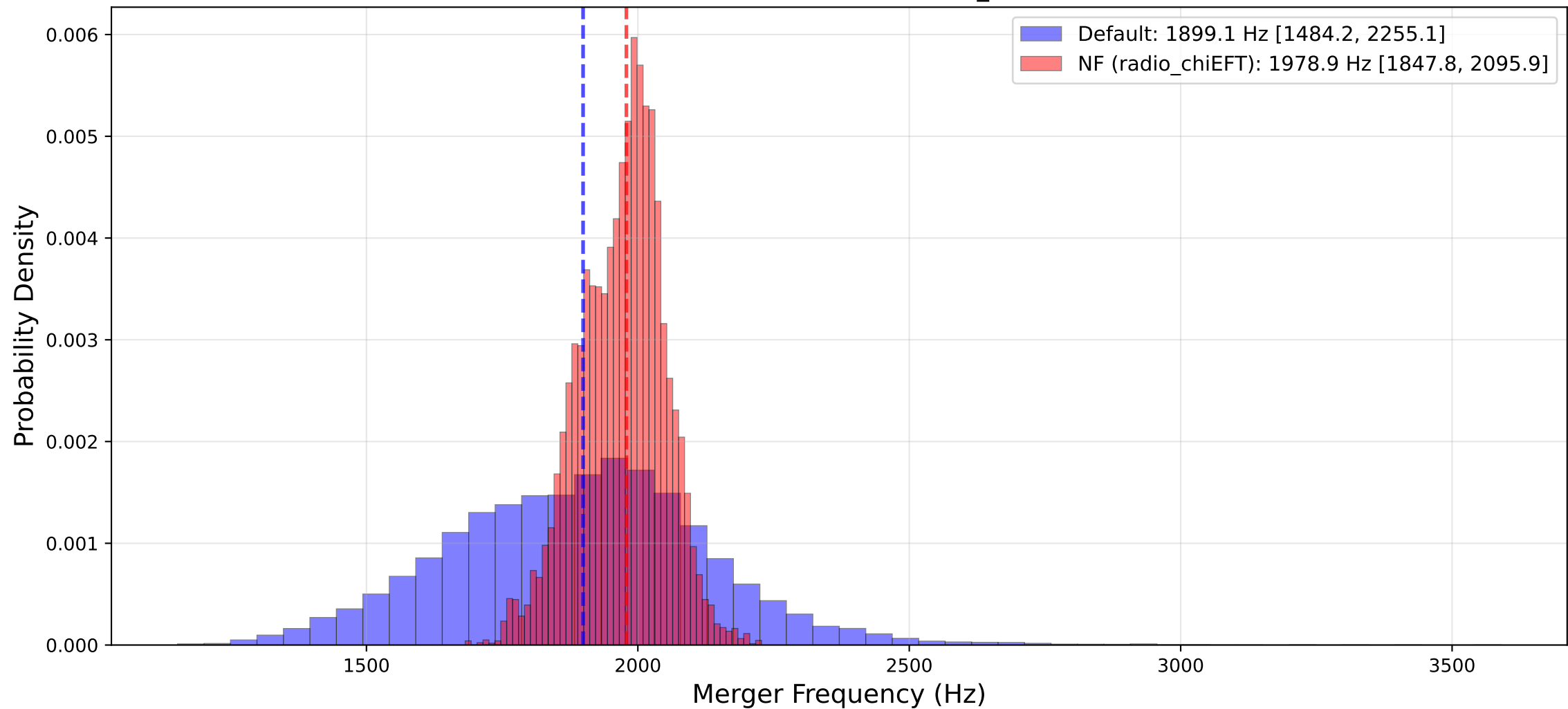
GW170817: NRTidalv3 Merger Frequency Comparison Default vs BNS Gaussian radio_chiEFT
