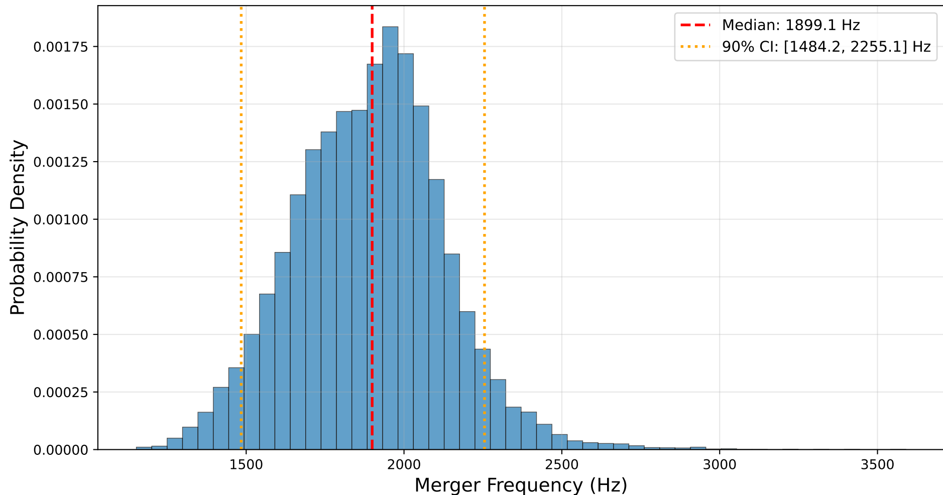
GW170817 Default (Agnostic Prior) NRTidalv3 Merger Frequency Distribution Median: 1899.1 Hz, 90% CI: [1484.2, 2255.1] Hz
