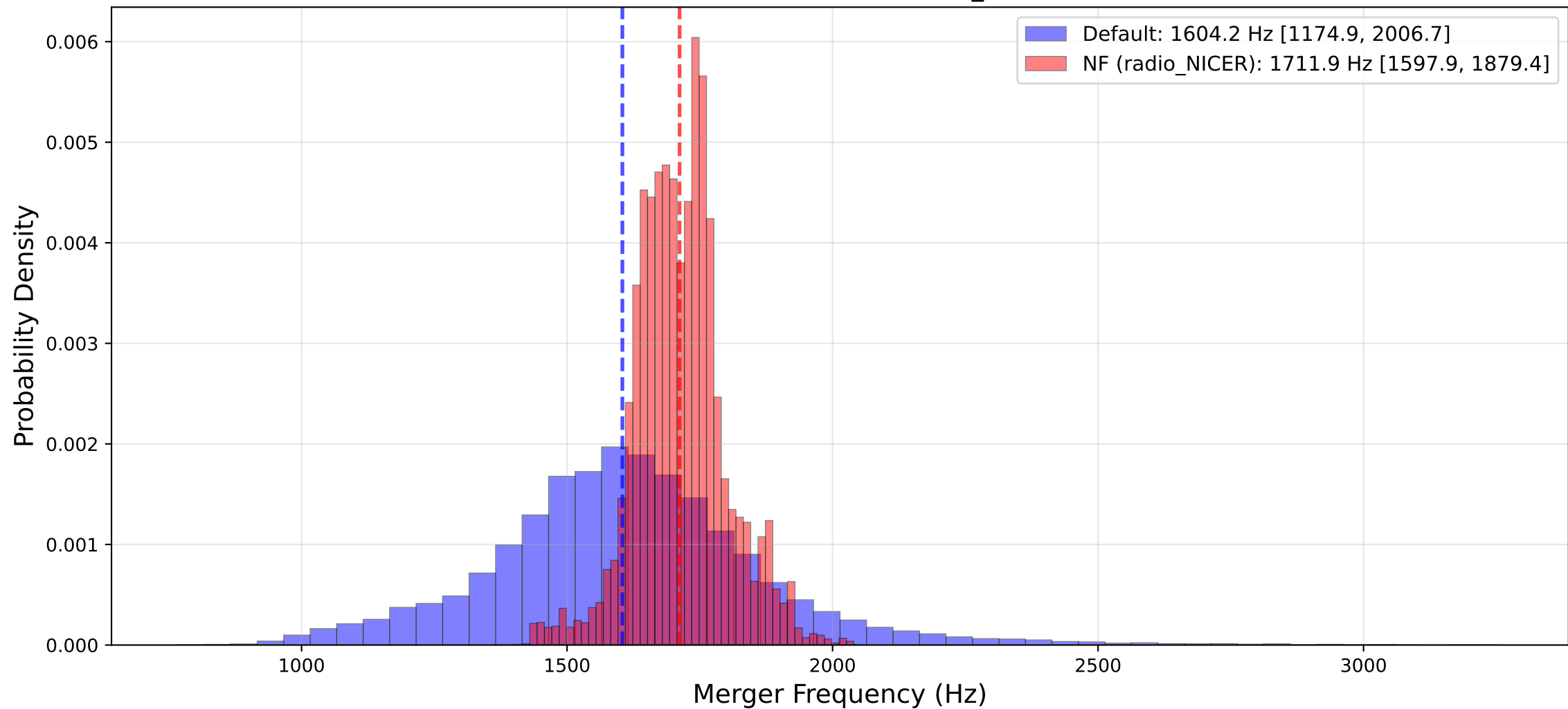
GW190425: NRTidalv3 Merger Frequency Comparison Default vs BNS uniform radio_NICER
