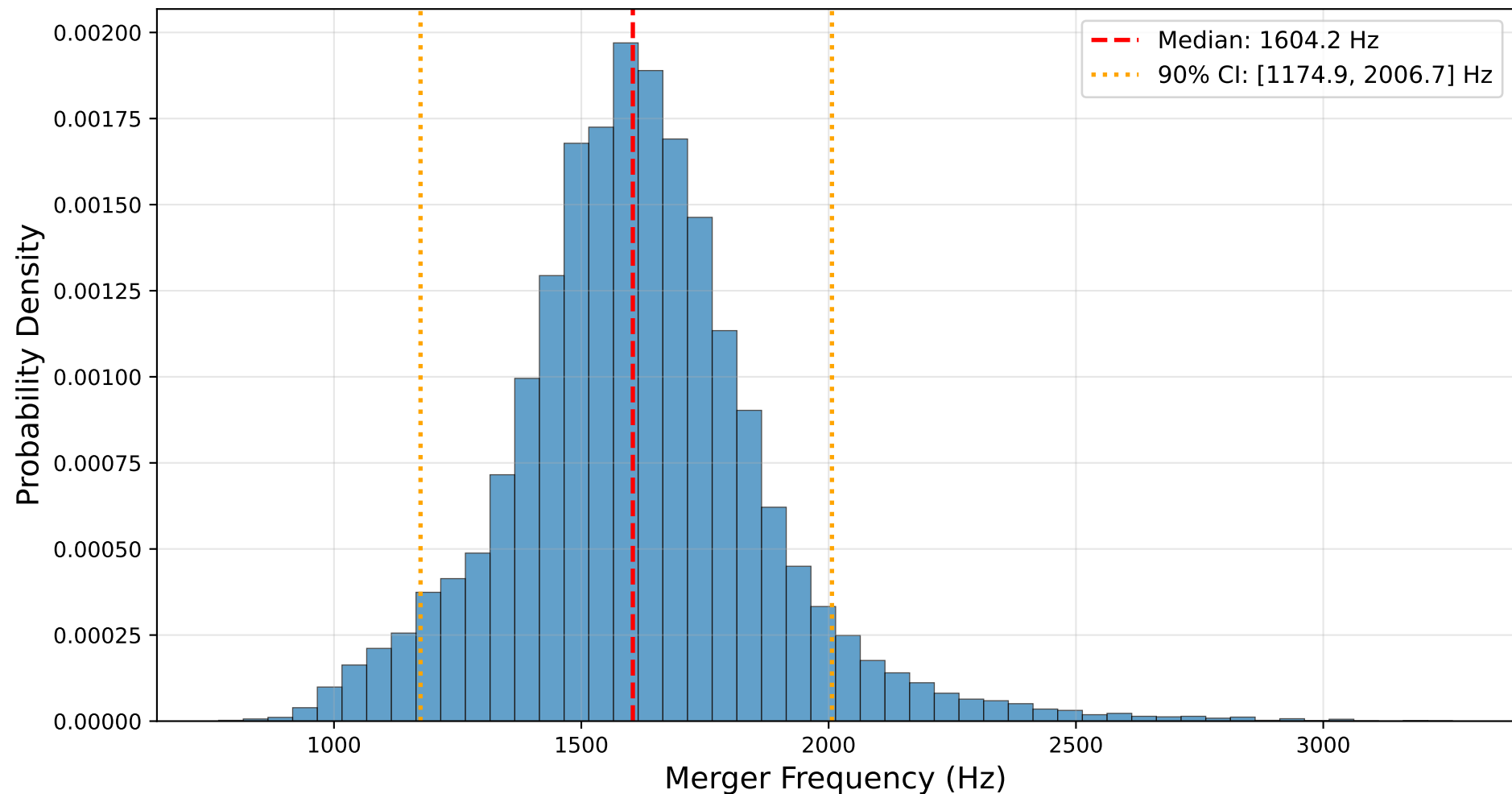
GW190425 Default (Agnostic Prior) NRTidalv3 Merger Frequency Distribution Median: 1604.2 Hz, 90% CI: [1174.9, 2006.7] Hz
