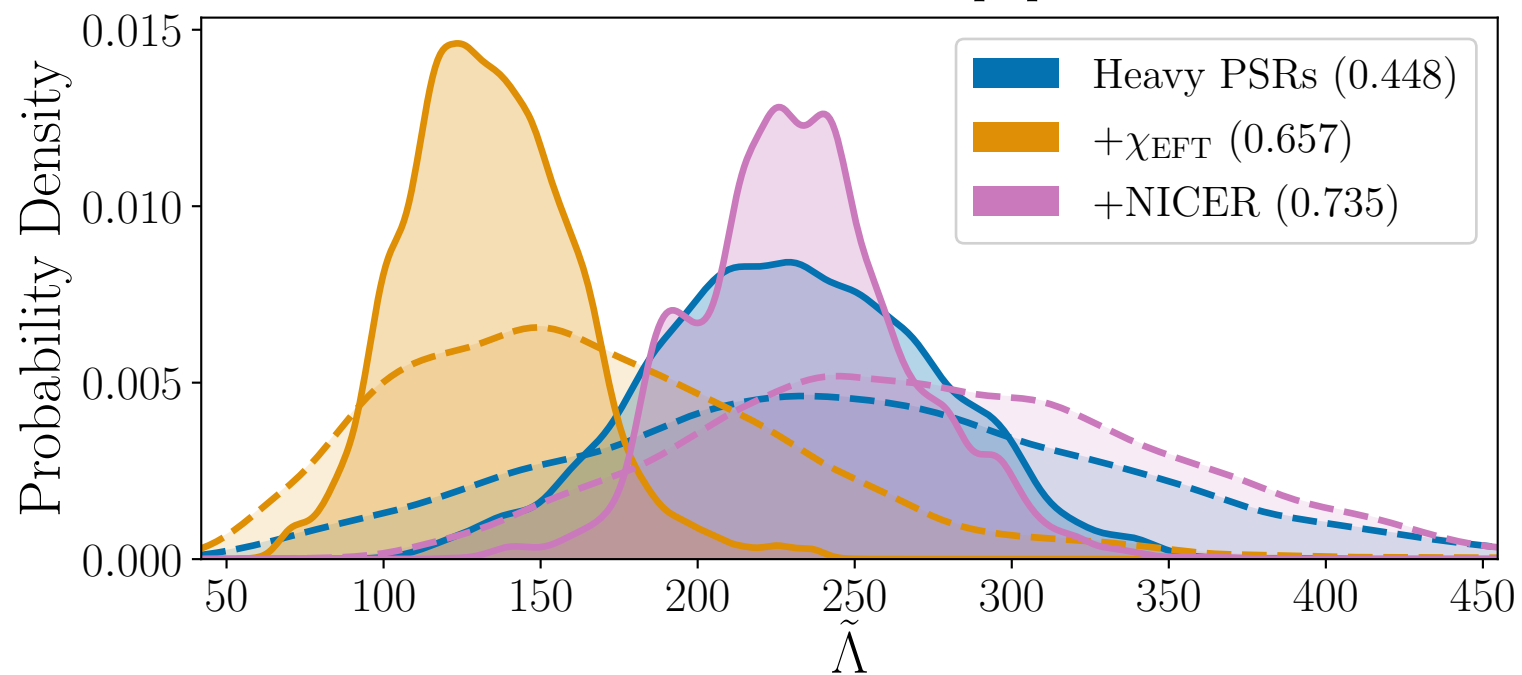
GW230529 - Gaussian population
