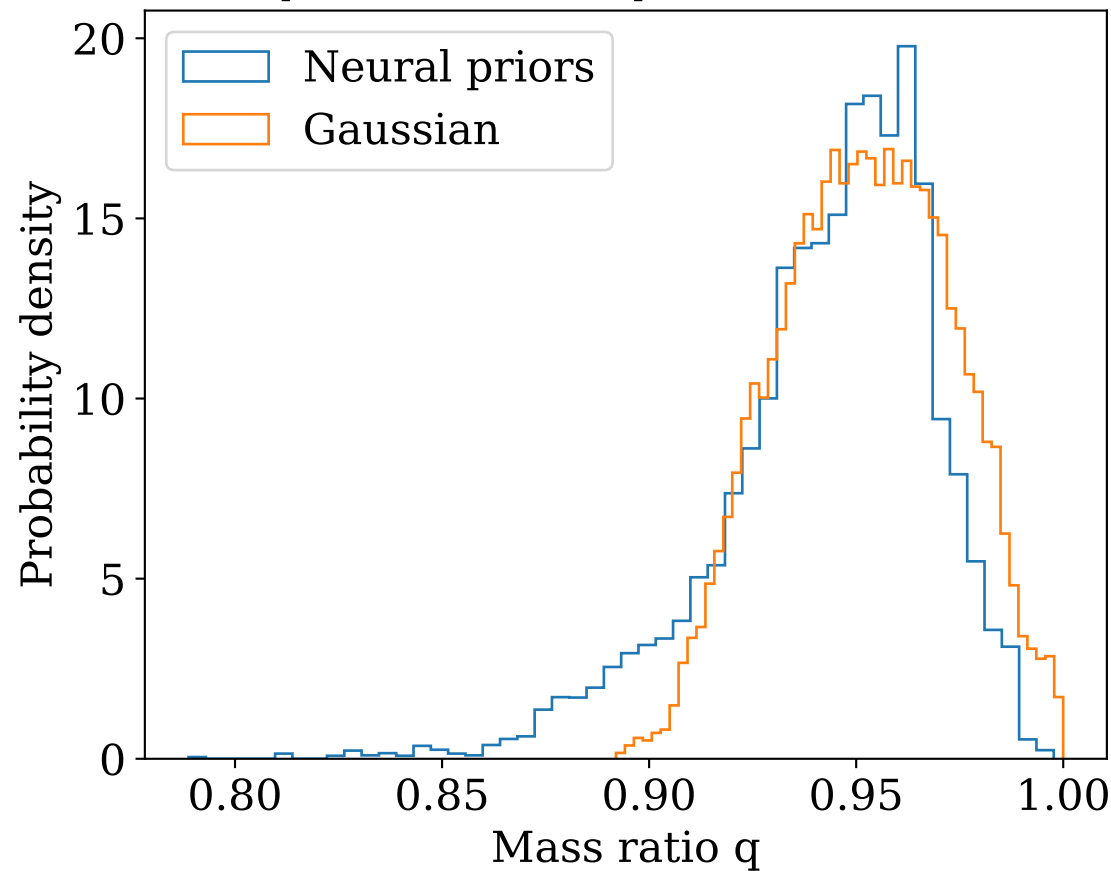
Comparison of mass ratio posteriors for GW170817
