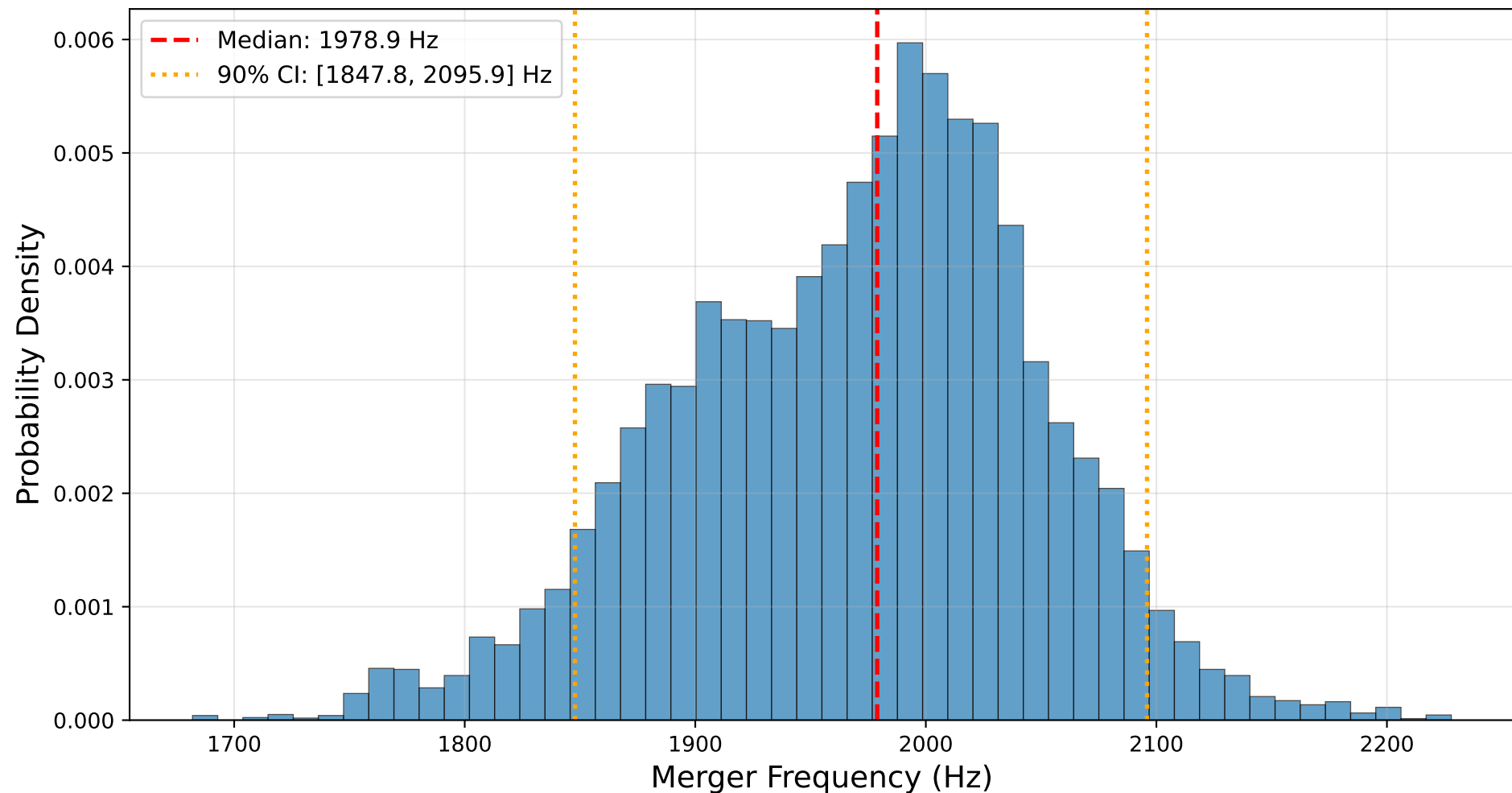
GW170817 BNS Gaussian radio_chiEFT NRTidalv3 Merger Frequency Distribution Median: 1978.9 Hz, 90% CI: [1847.8, 2095.9] Hz
