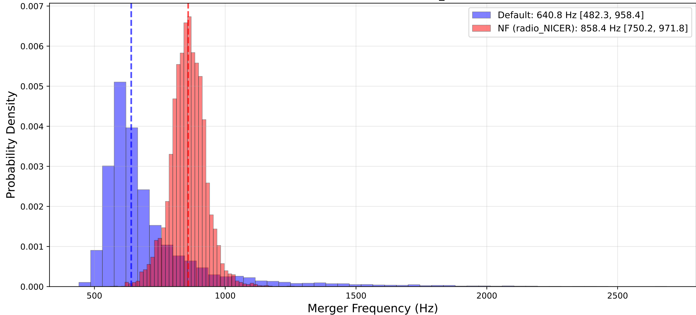
GW230529: NRTidalv3 Merger Frequency Comparison Default vs NSBH Gaussian radio_NICER
