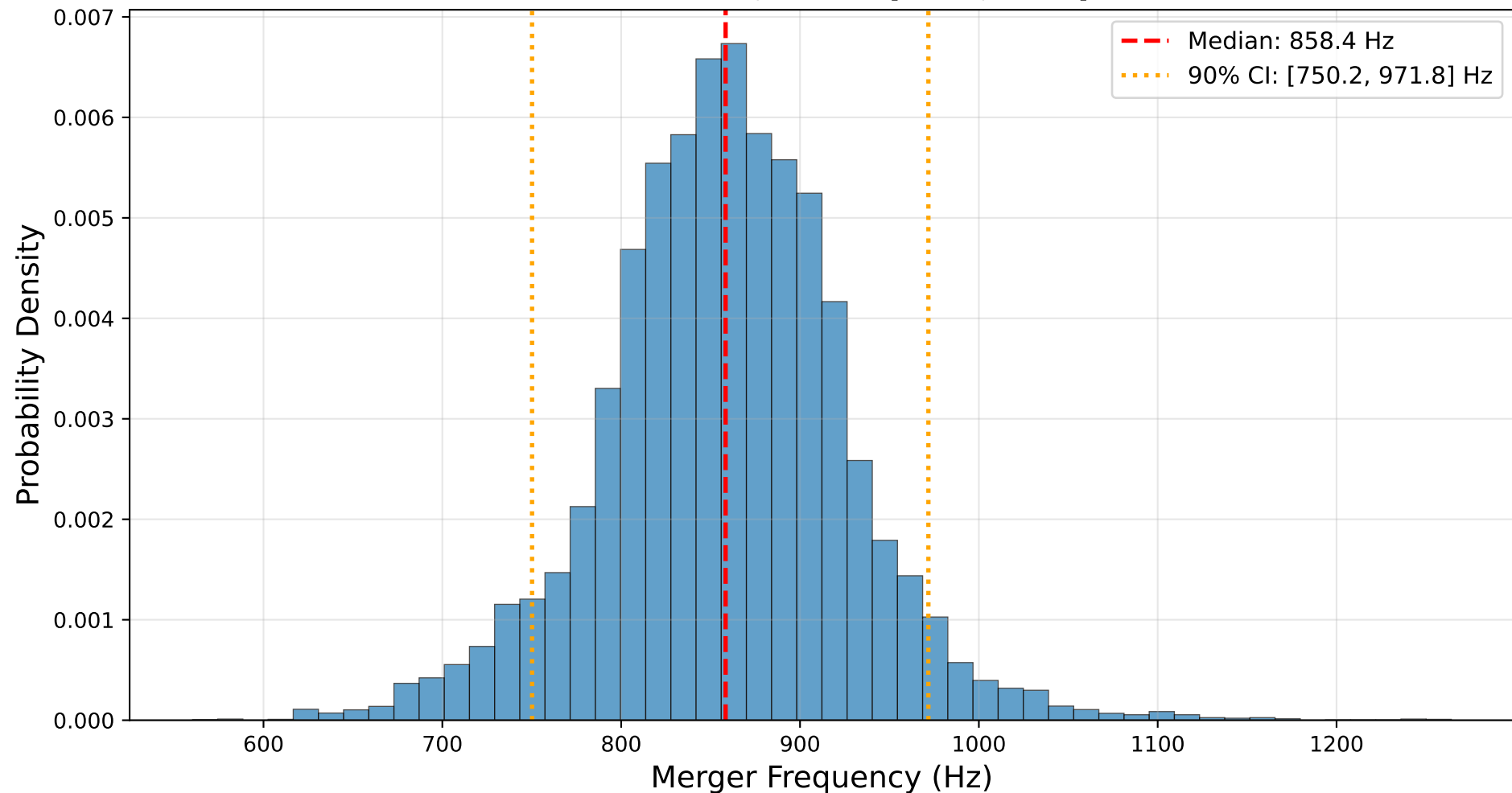
GW230529 NSBH Gaussian radio_NICER NRTidalv3 Merger Frequency Distribution Median: 858.4 Hz, 90% CI: [750.2, 971.8] Hz
