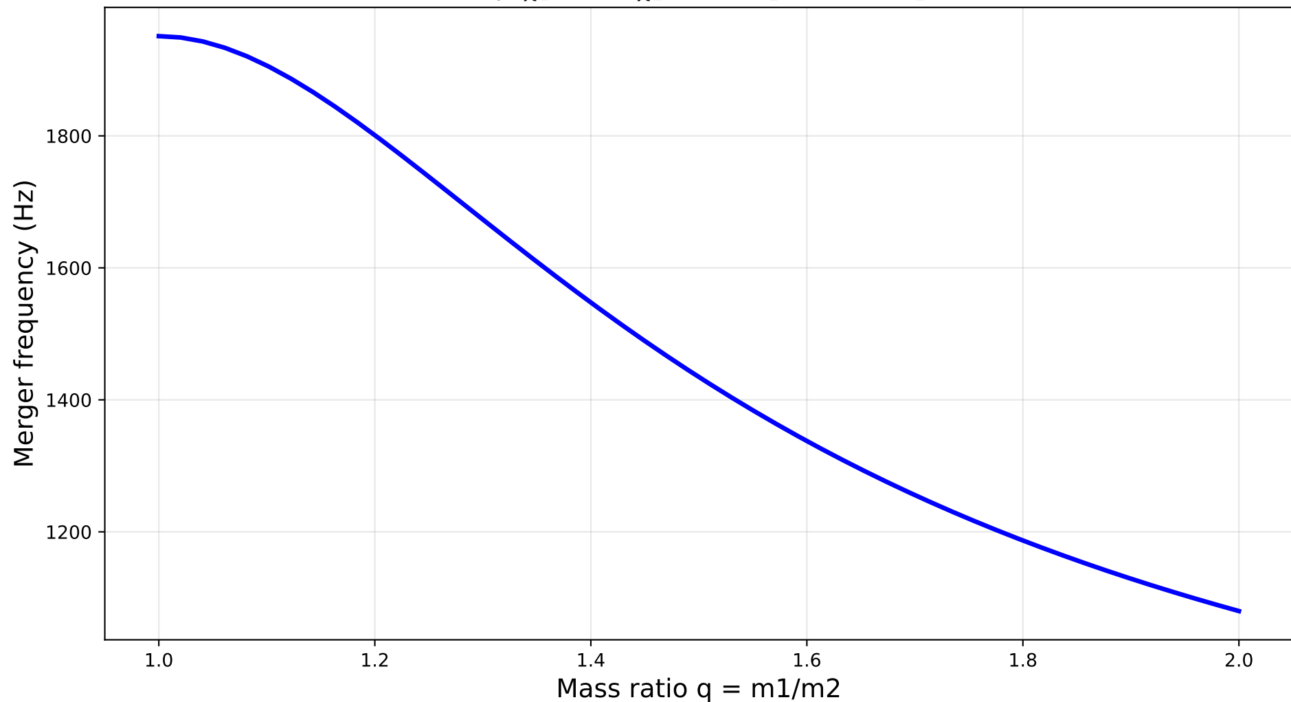
GW170817: NRTidalv3 Merger Frequency vs Mass Ratio ( M = 2.8 M_{\odot} , \chi_1 = 0.0 , \chi_2 = 0.0 , \Lambda_1 = 400.0 , \Lambda_2 = 400.0 )
