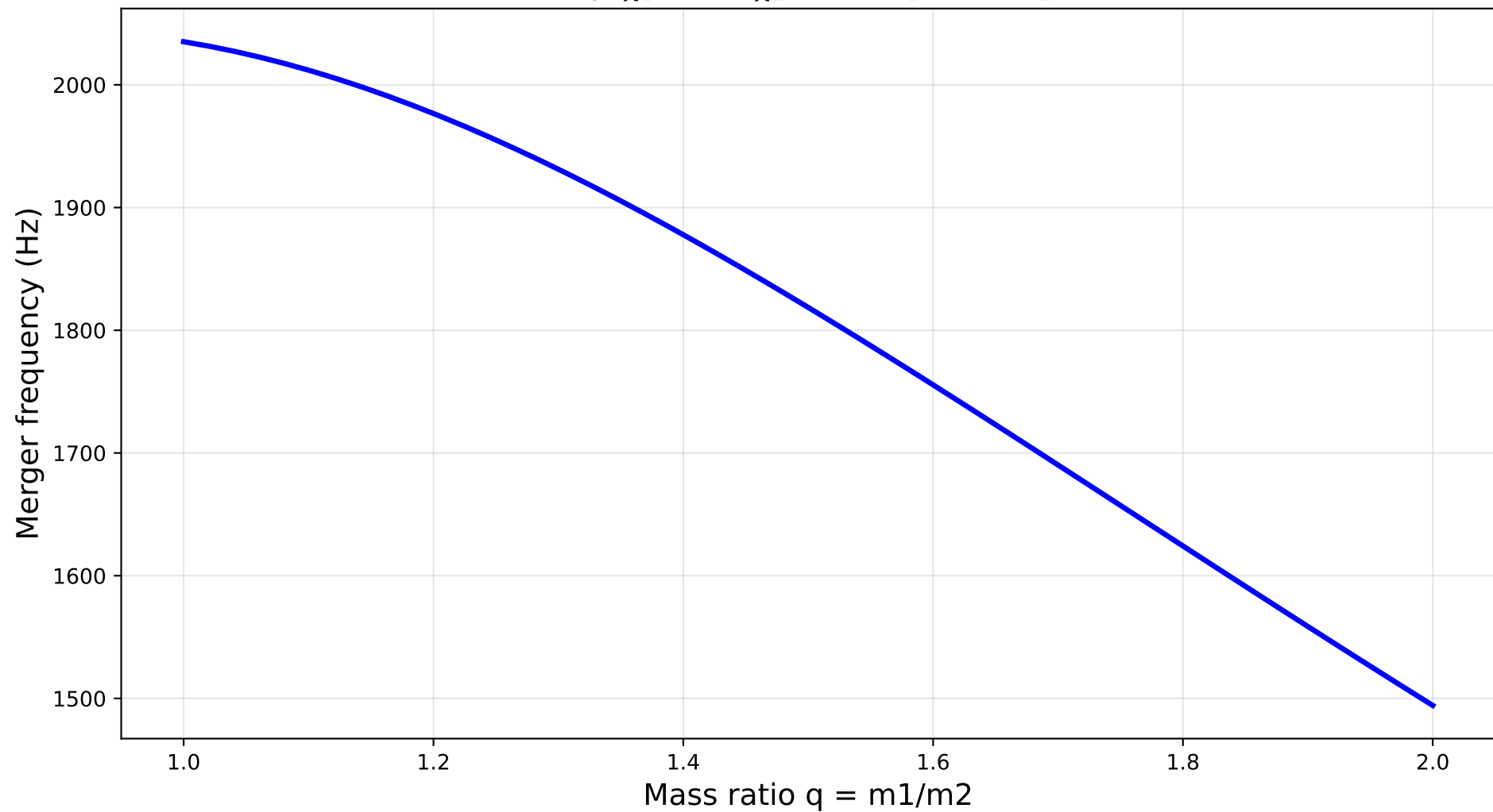
GW230529: NRTidalv3 Merger Frequency vs Mass Ratio ( M = 5.0 M_{\odot} , \chi_1 = 0.0 , \chi_2 = 0.0 , \Lambda_1 = 0.0 , \Lambda_2 = 400.0 )
