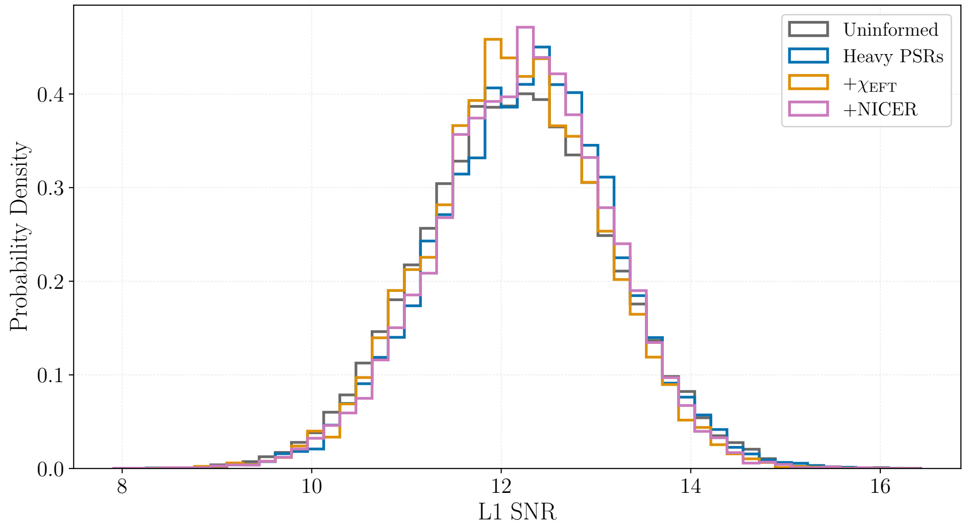
GW190425 - Uniform Population
