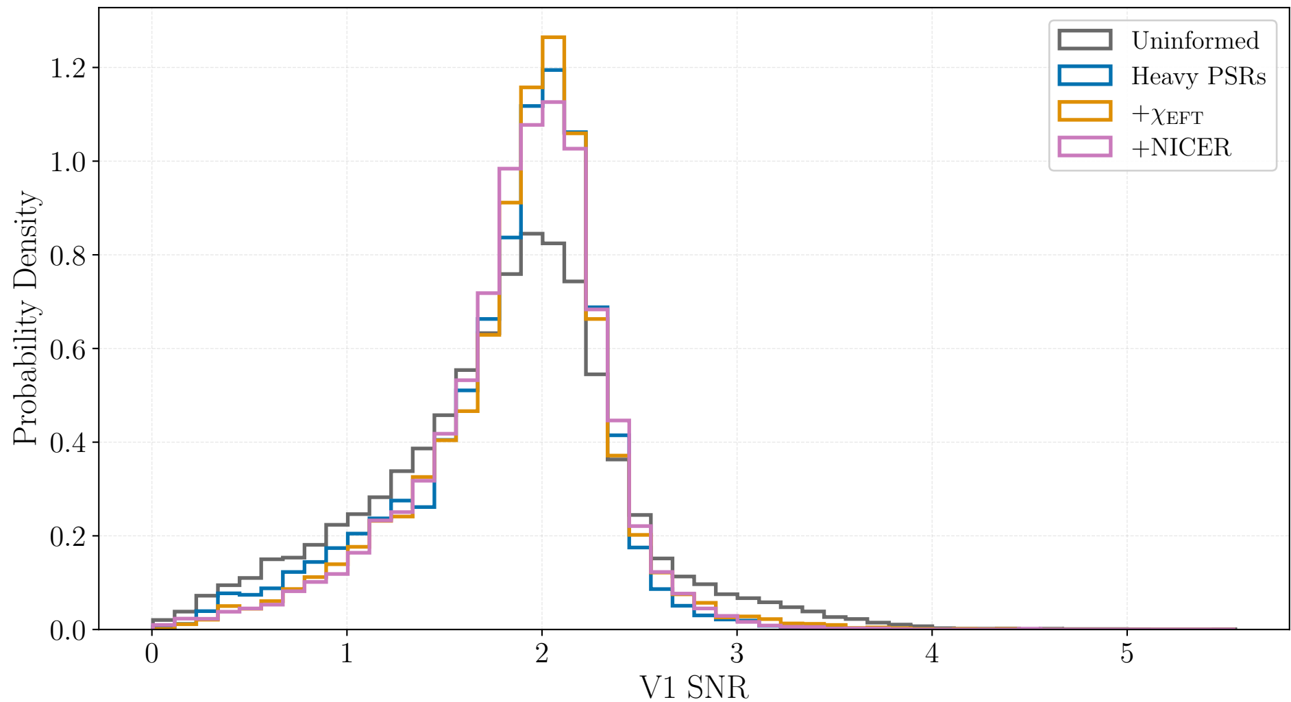
GW190425 - Double Gaussian Population
