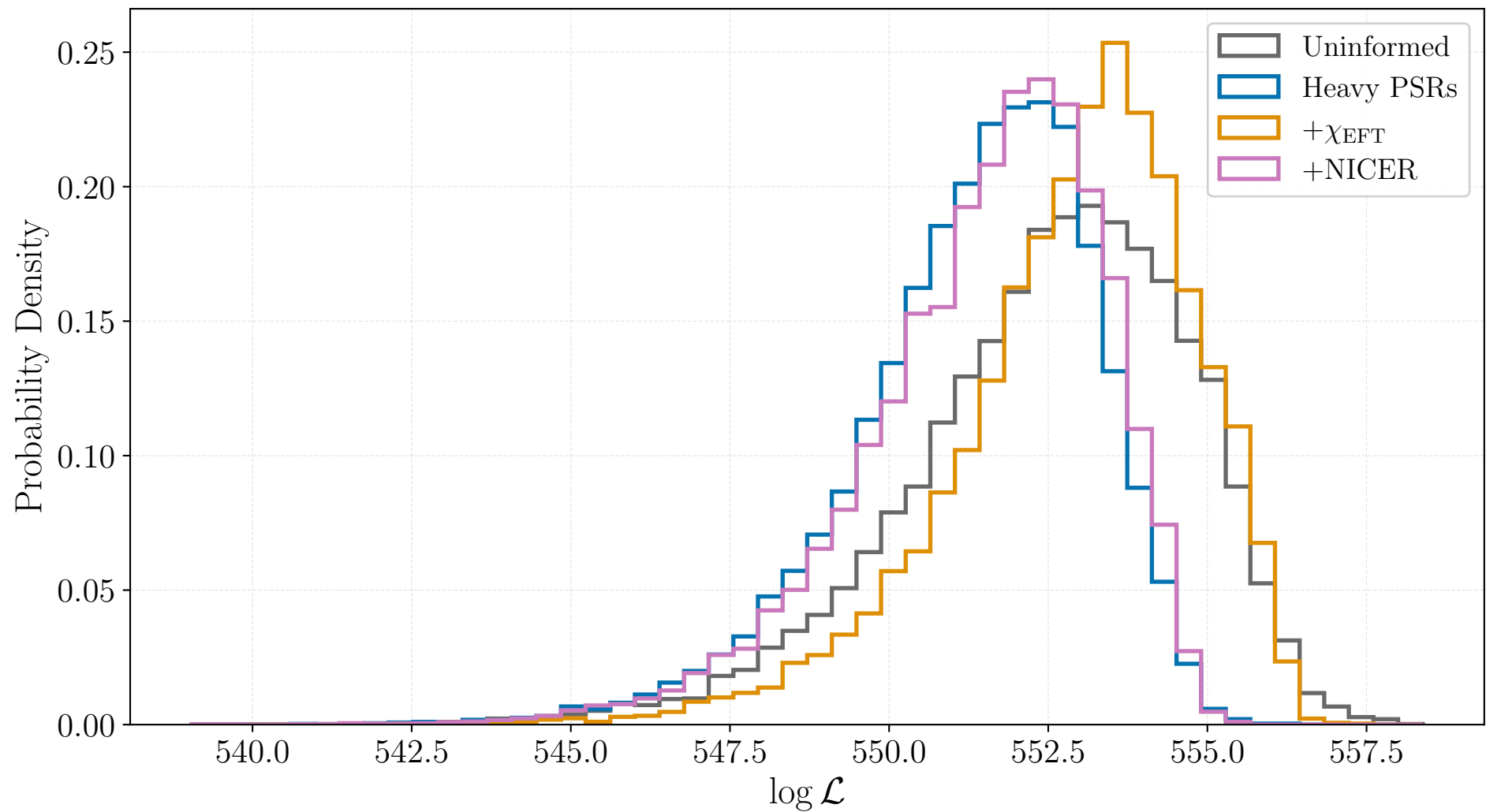
GW170817 - Double Gaussian Population
