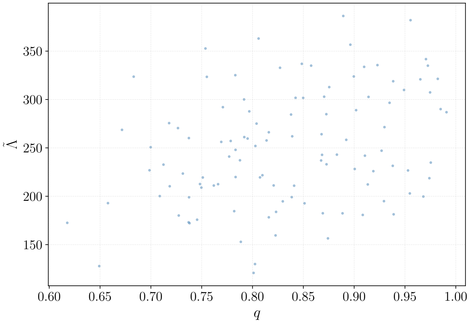
GW170817 BNS Default ( \log L_{\text{ch}} 556.8 )
