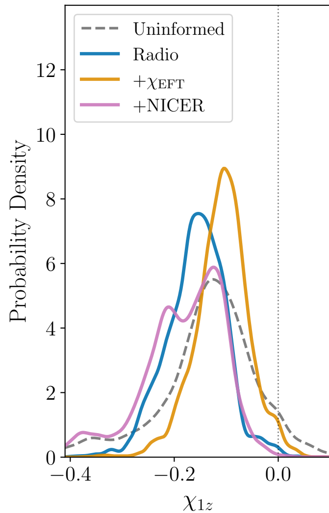
Uniform
