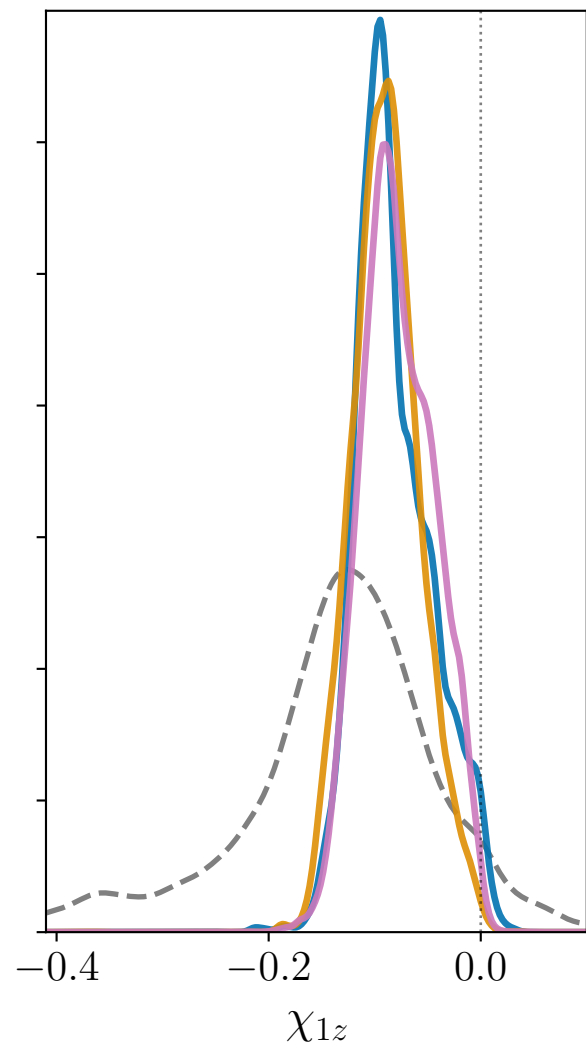
Double Gaussian
