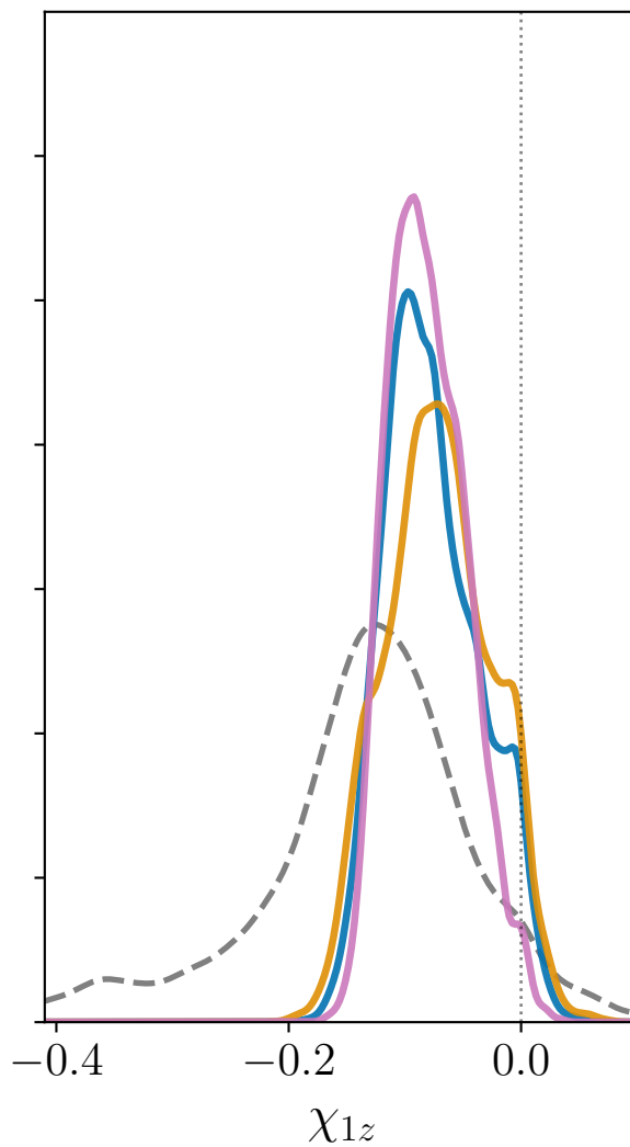
Gaussian
