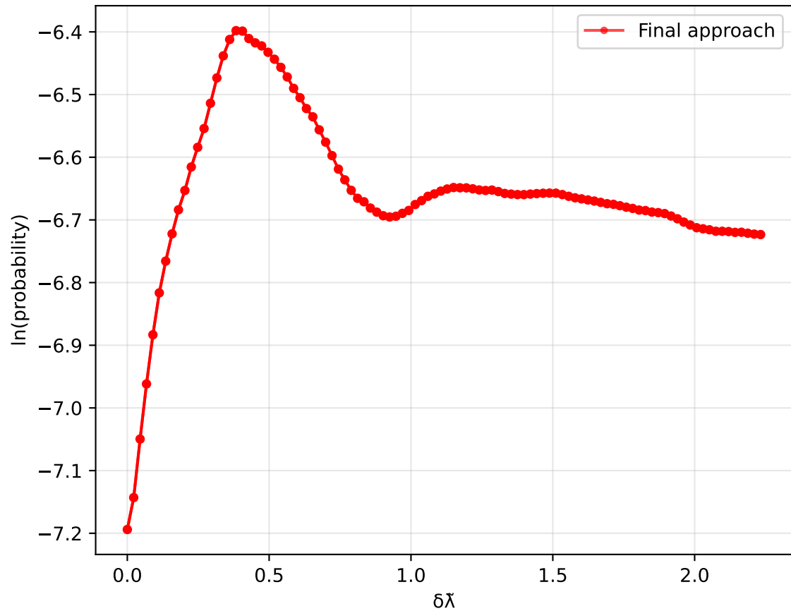
Approach to \delta\lambda=0 ( \lambda_1=\lambda_2 )
