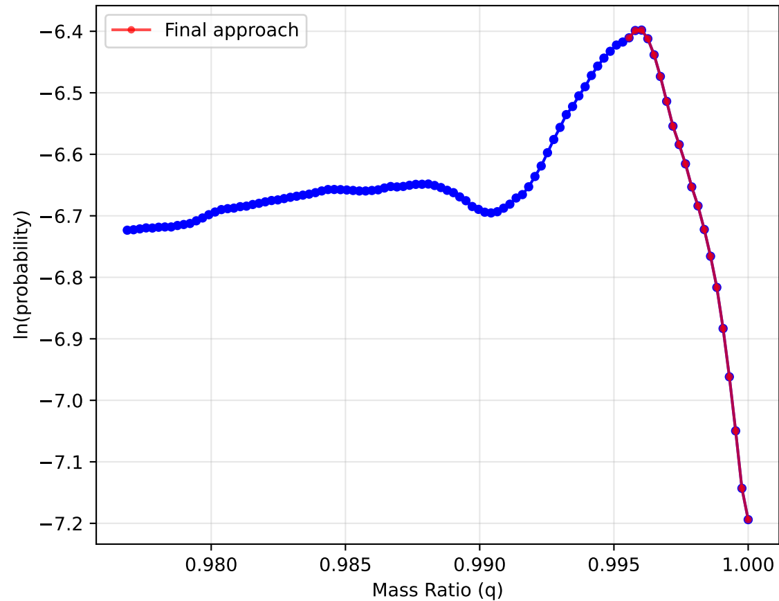
Approach to q=1 Boundary
