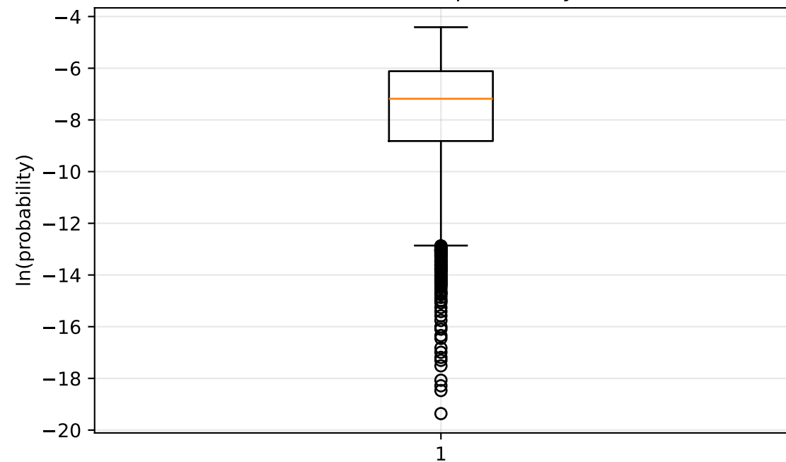
Box Plot of \ln(\text{probability})
