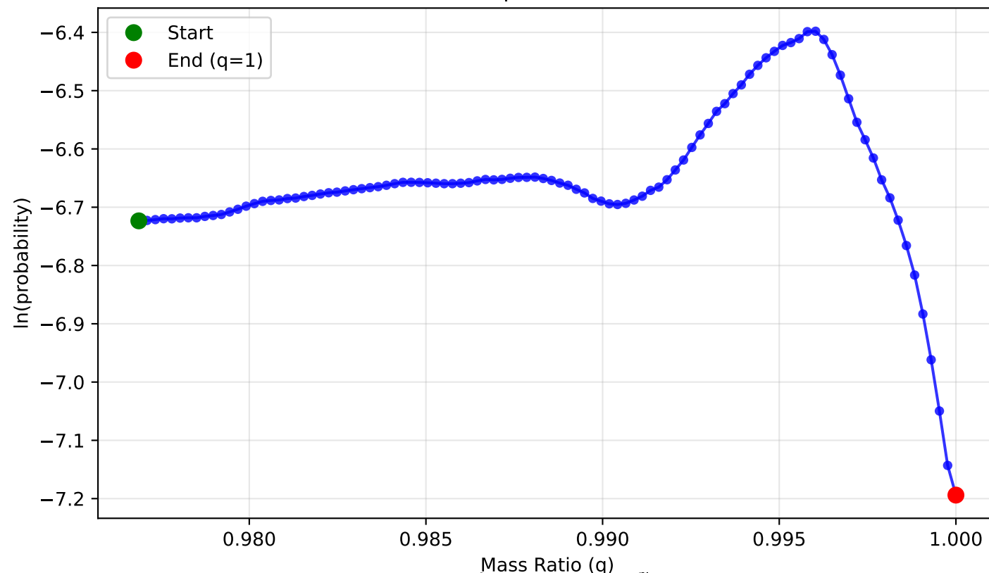
NF Prior: \ln(\text{prob}) vs Mass Ratio
