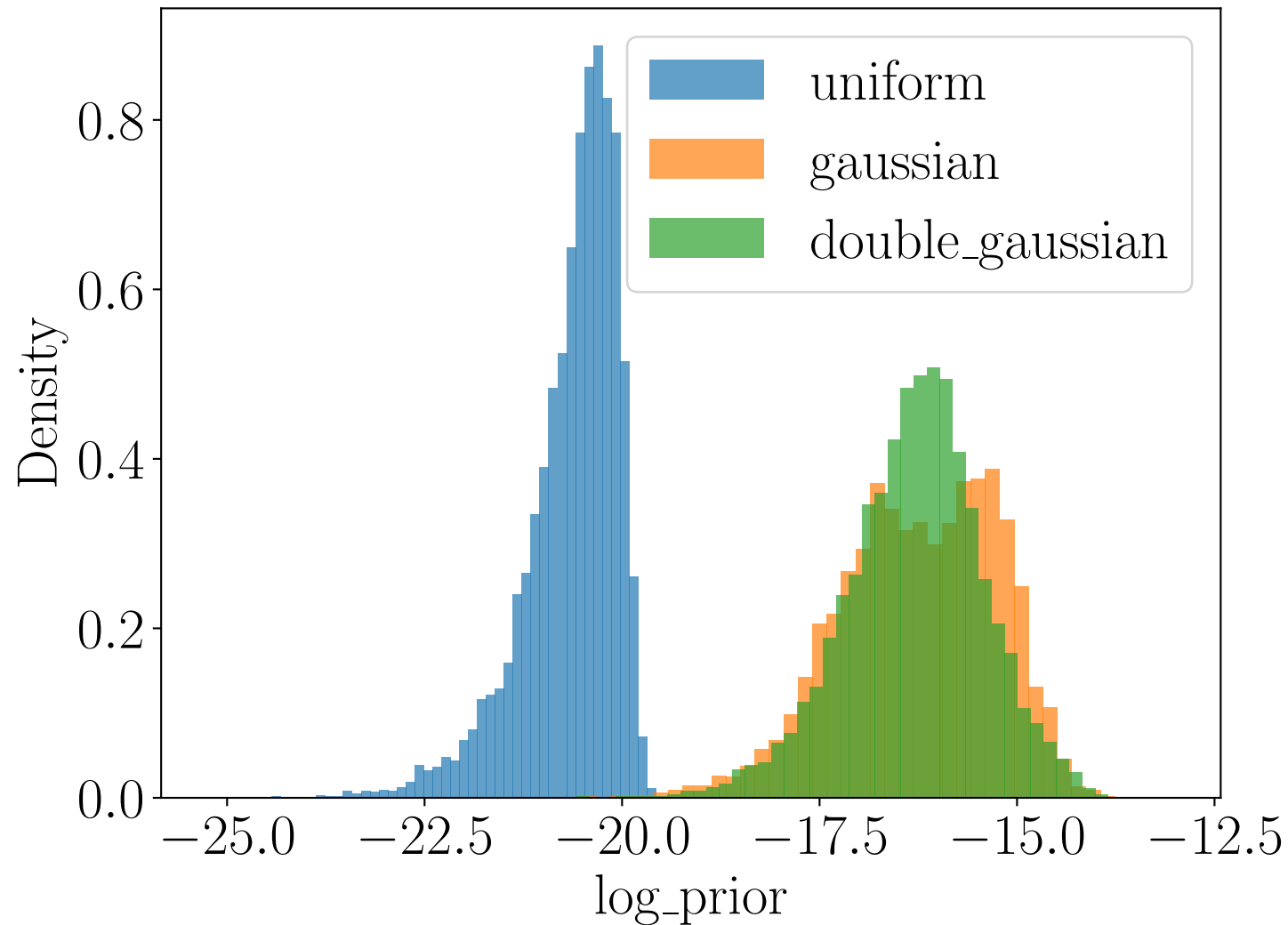
Distribution of log_prior values
