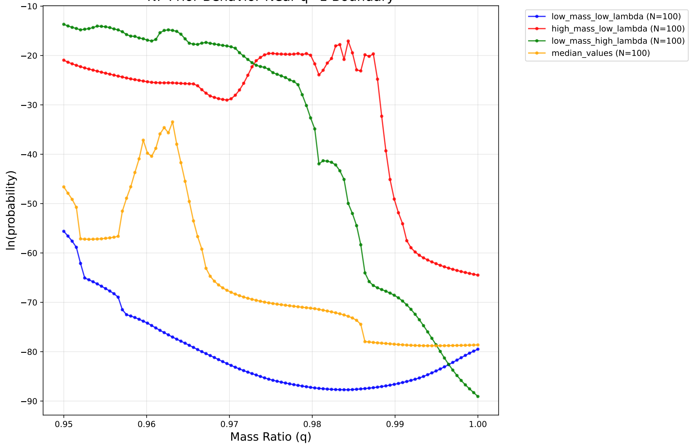
NF Prior Behavior Near q=1 Boundary
