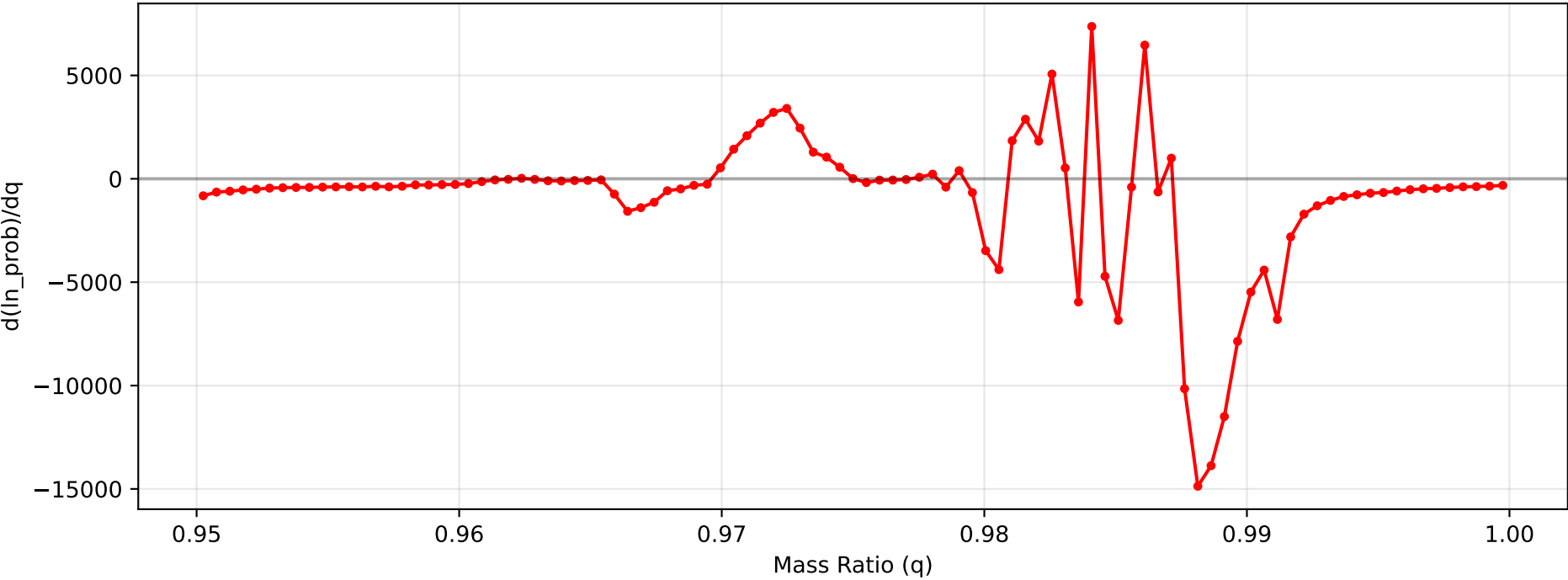
Approximate Derivative
