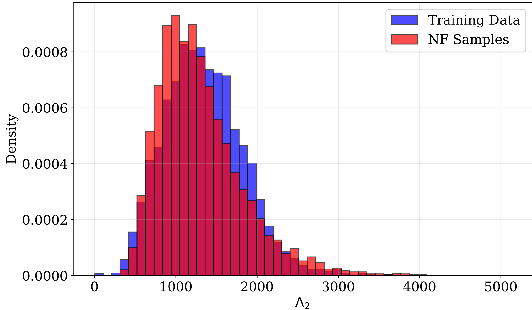
NSBH Conditional Prior: p(\Lambda_2|m_2 = 1.2M_\odot)
