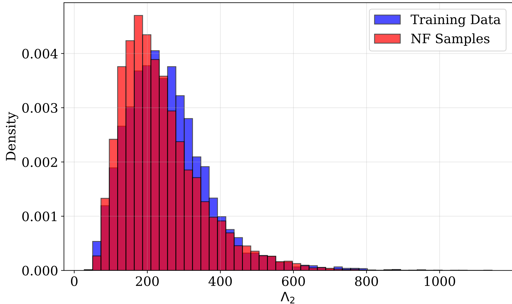
NSBH Conditional Prior: p(\Lambda_2|m_2 = 1.6M_\odot)
