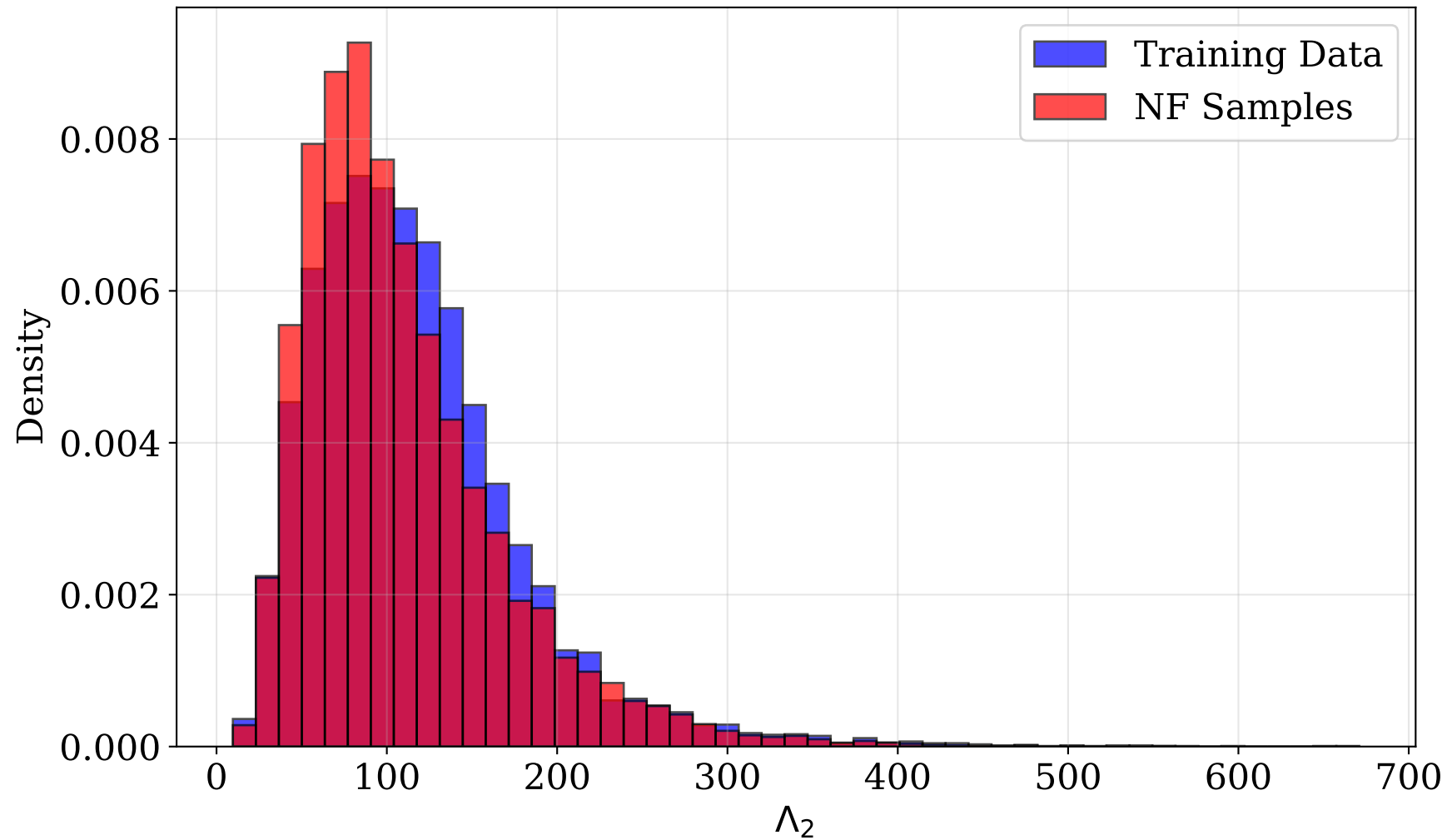
NSBH Conditional Prior: p(\Lambda_2|m_2 = 1.8M_\odot)
