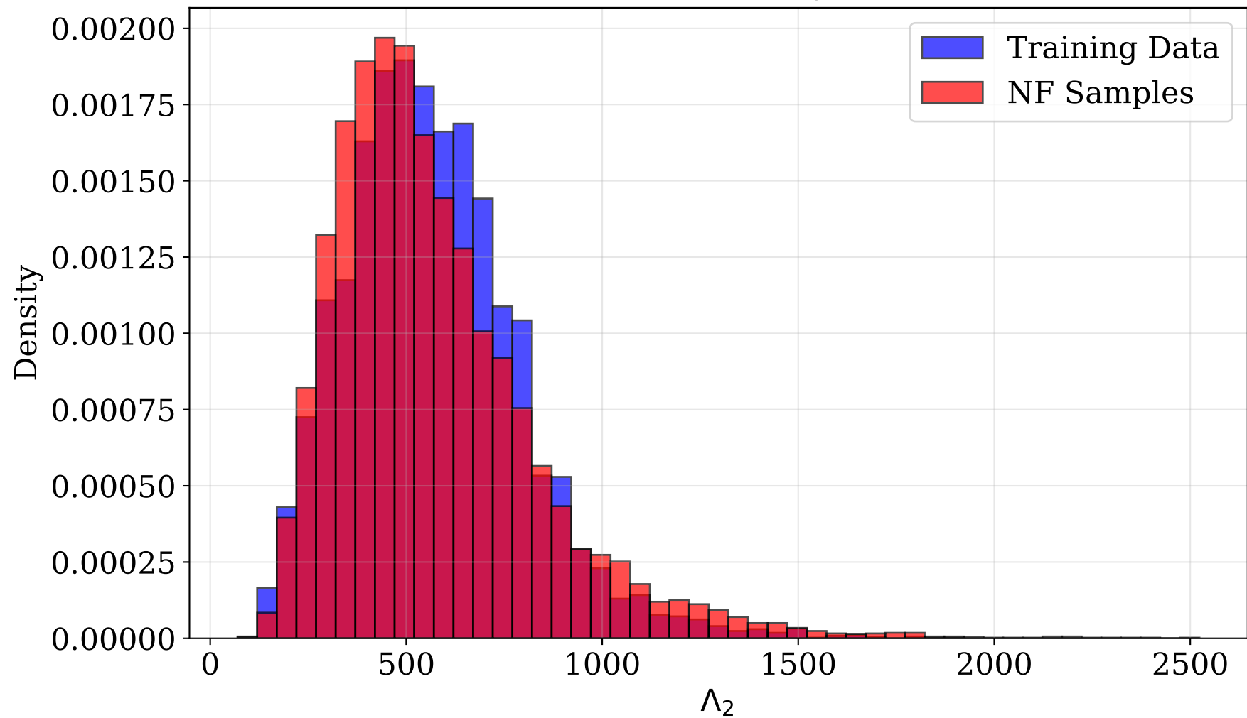
NSBH Conditional Prior: p(\Lambda_2|m_2 = 1.4M_\odot)
