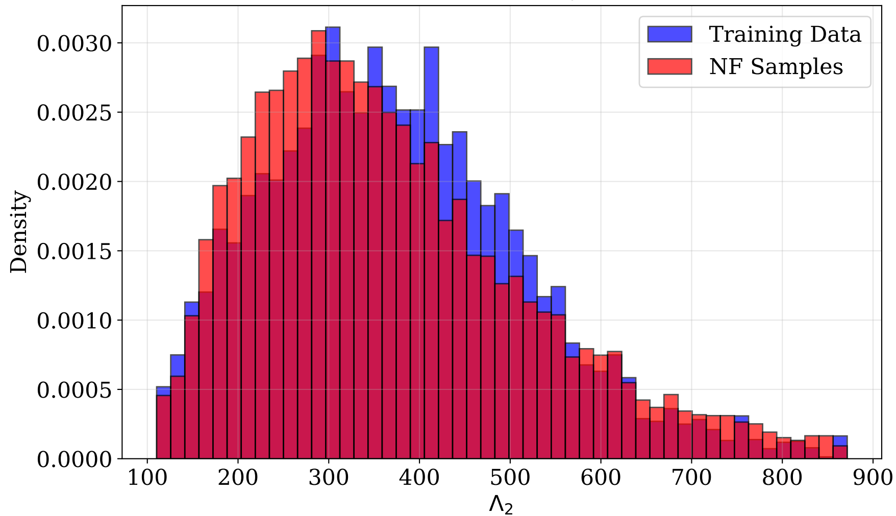
NSBH Conditional Prior: p(\Lambda_2|m_2 = 1.5M_\odot)
