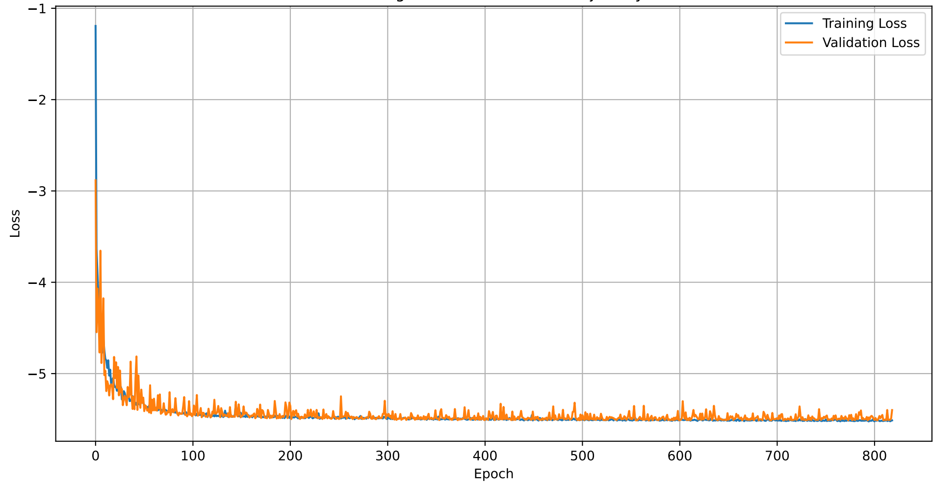
Training and Validation Loss Trajectory
