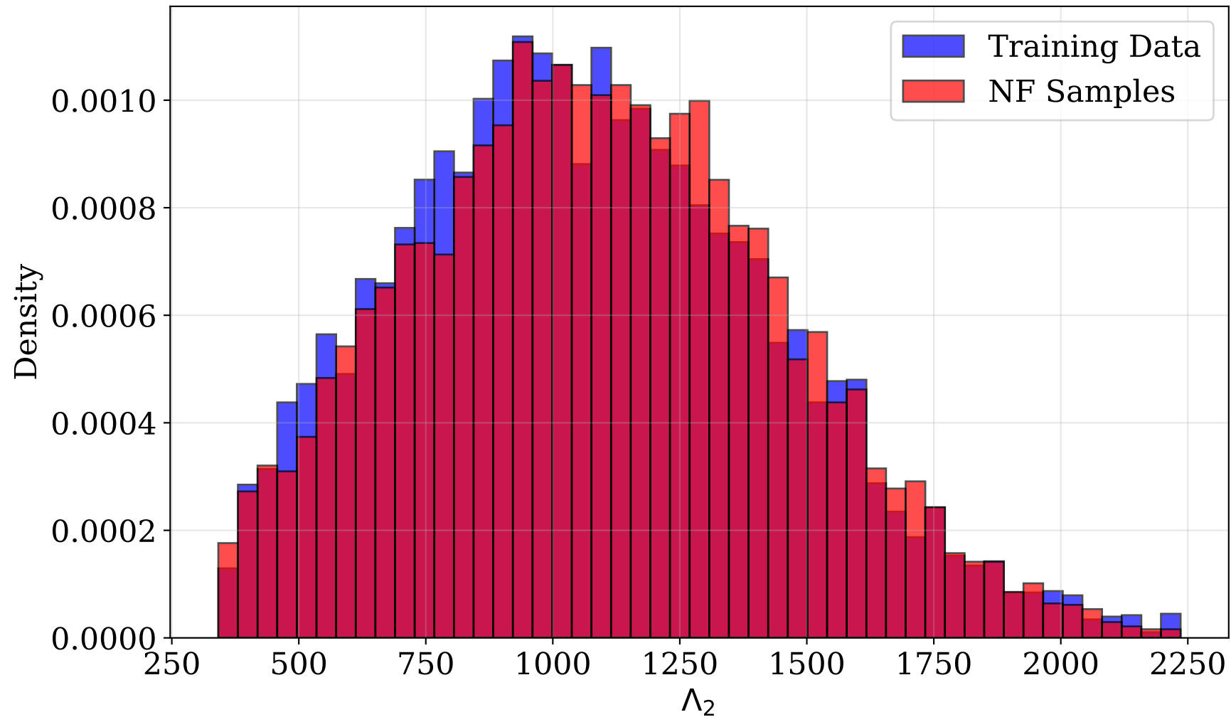
NSBH Conditional Prior: p(\Lambda_2|m_2 = 1.2M_\odot)
