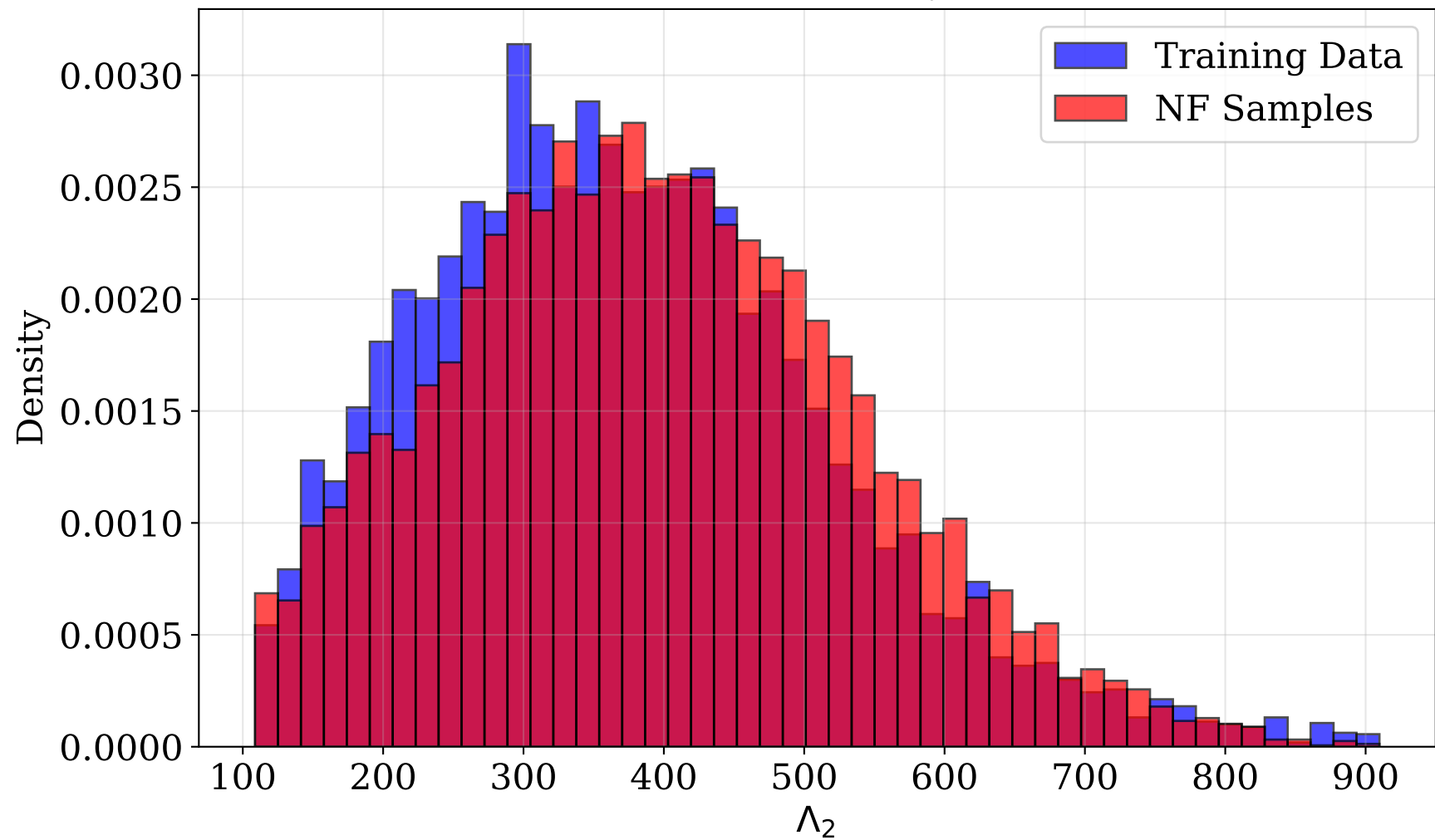
NSBH Conditional Prior: p(\Lambda_2|m_2 = 1.5M_\odot)
