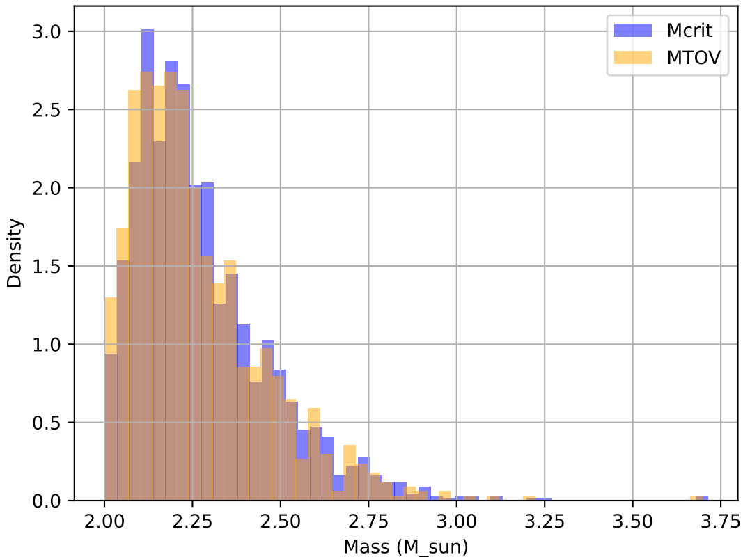
Histogram of Mcrit and MTOV
