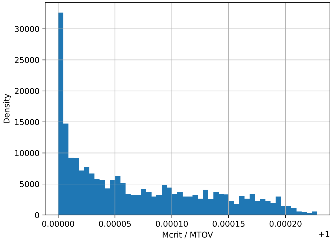
Histogram of Mcrit / MTOV ratios
