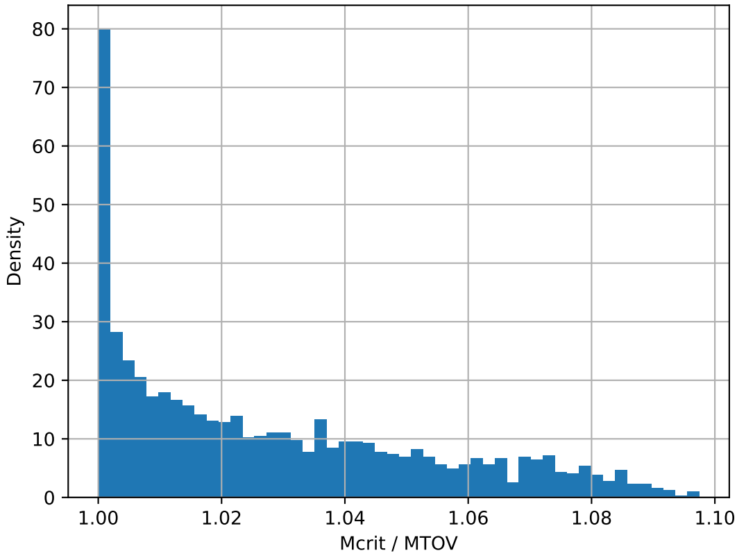
Histogram of M_{\text{crit}} / M_{\text{TOV}} ratios
