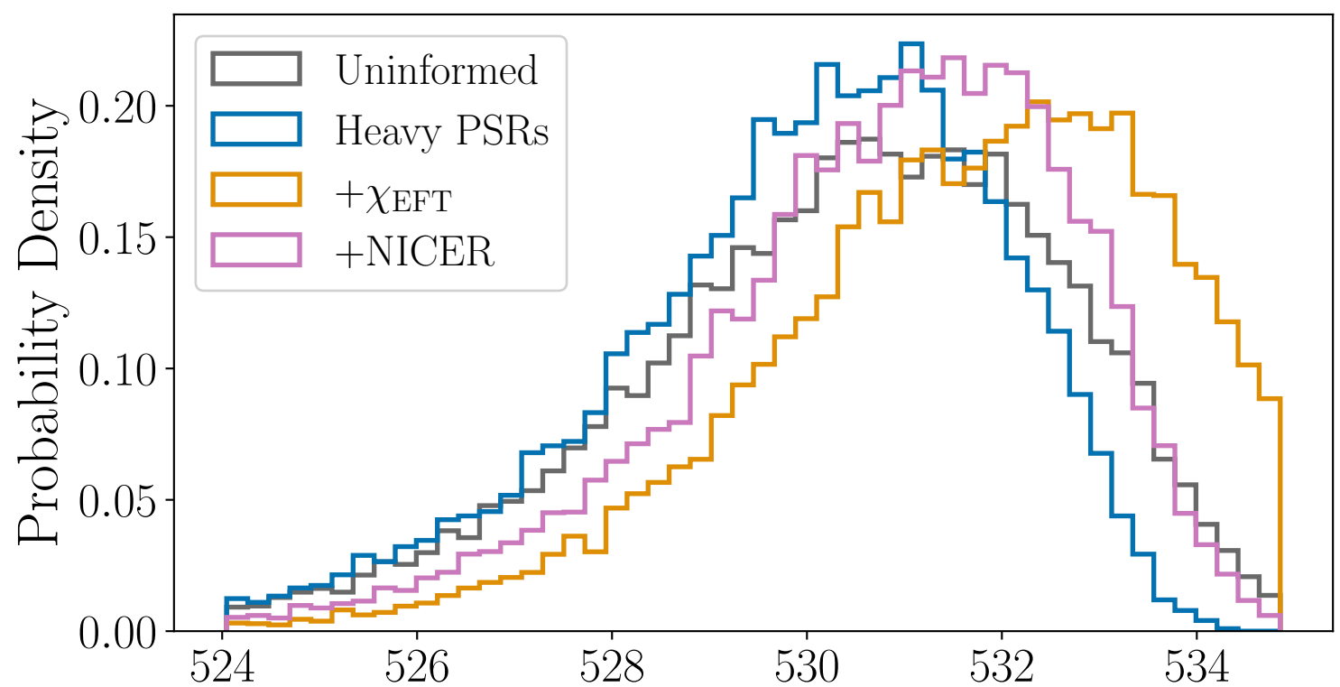
GW190425 - Uniform population (BNS)
