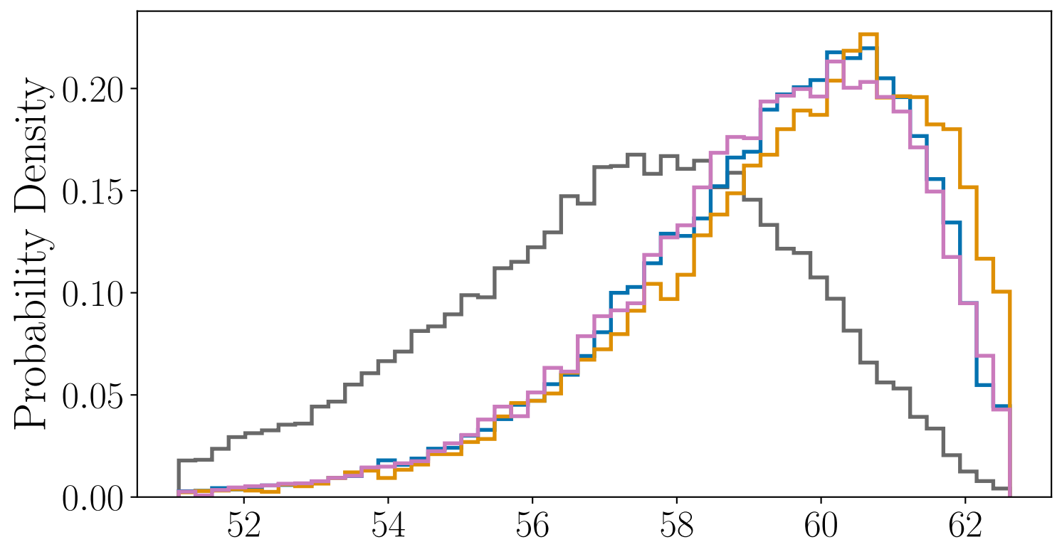
GW230529 - Gaussian population (NSBH)
