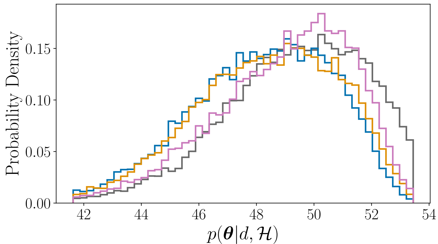
GW230529 - Gaussian population (NSBH)
