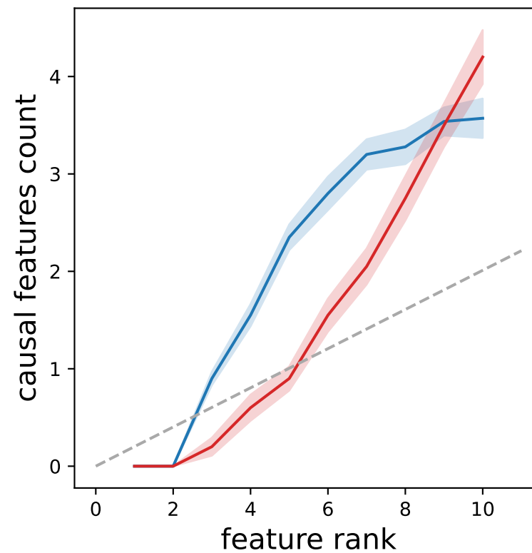
diabetes readmission
