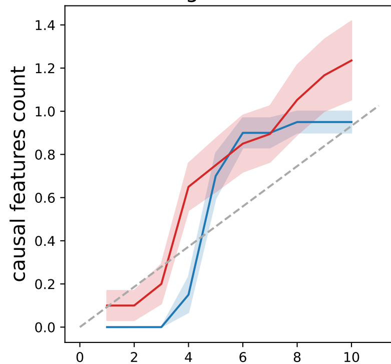
college scorecard
