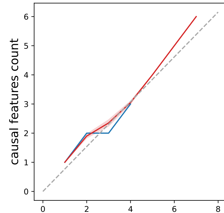
assistments
