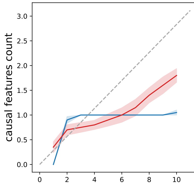
acsincome
