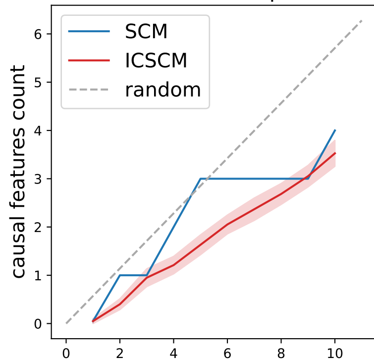
acsfoodstamps
