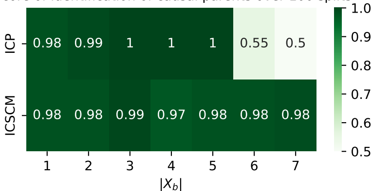
Recall score of identification of causal parents over 100 splits
