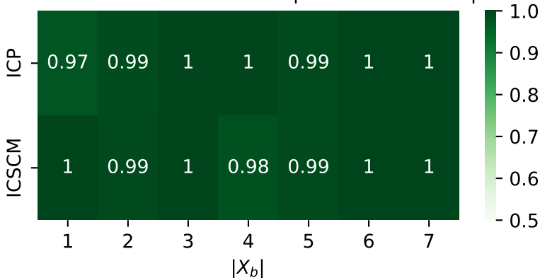
Precision score of identification of causal parents over 100 splits
