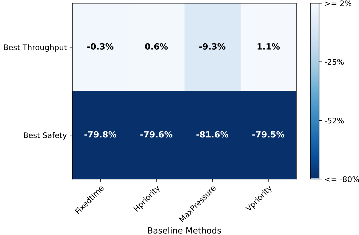
Throughput Improvement vs Baselines (Outflow %)
