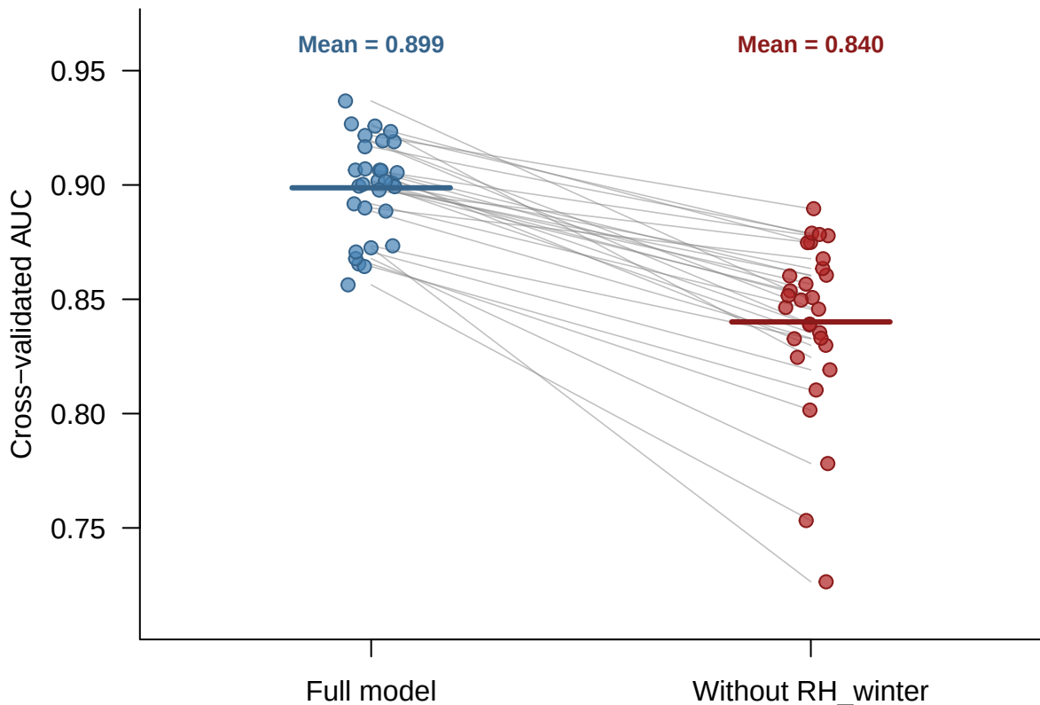
Paired AUC: full model vs model without relative_humidity_winter
